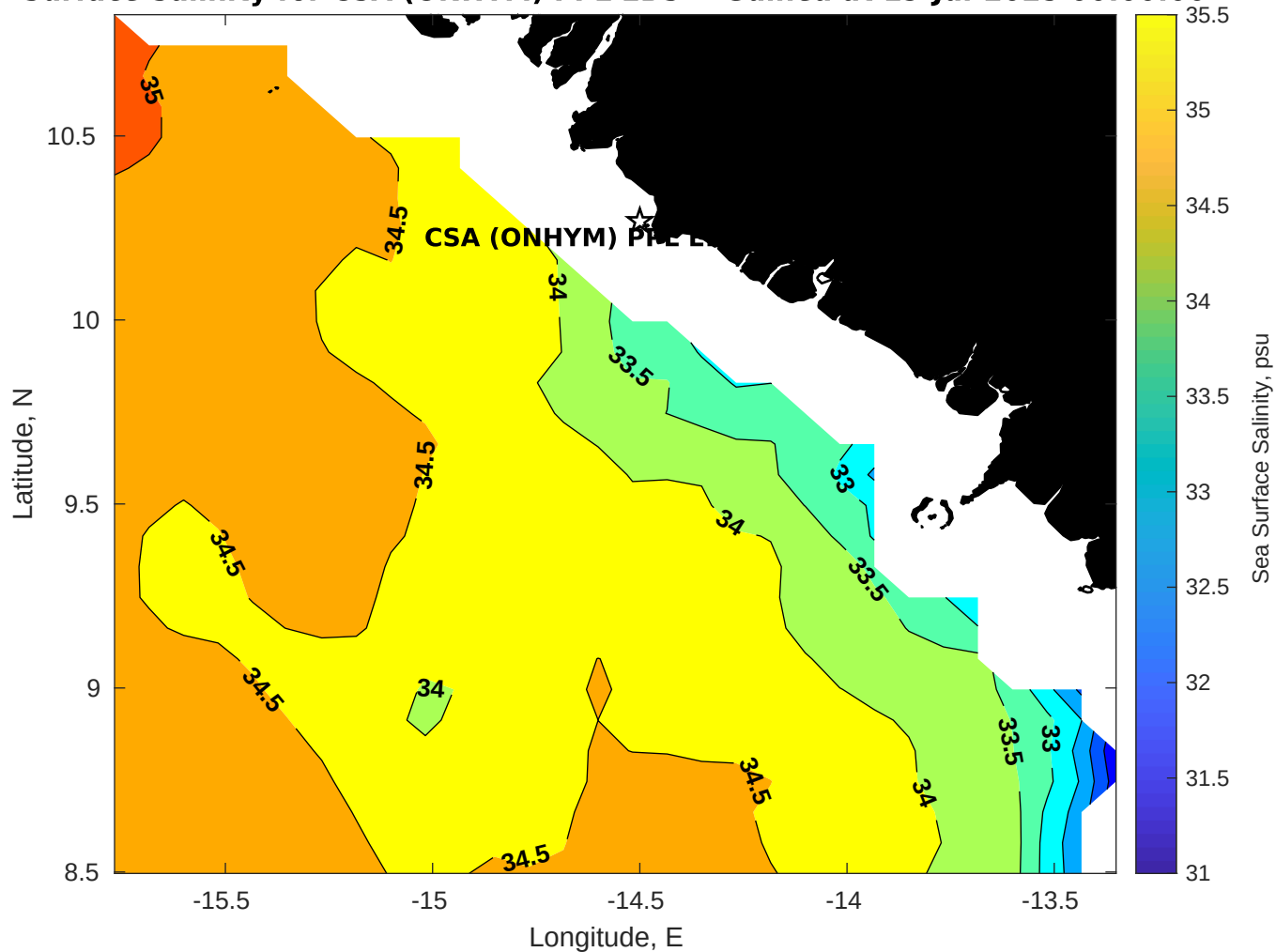
Surface Salinity for CSA (ONHYM) PPL EBS - Guinea at 19-Jul-2025 00:00:00
