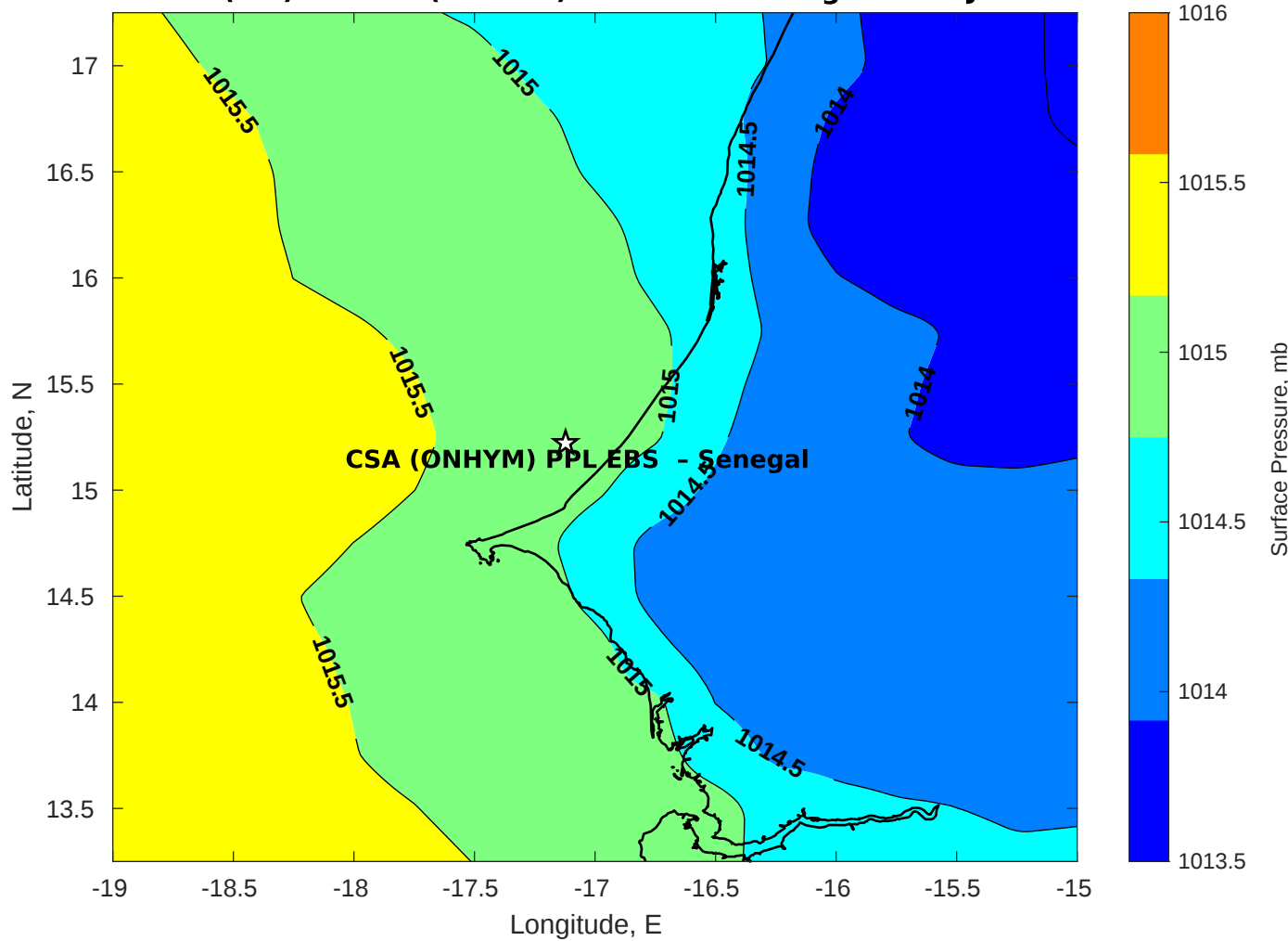
Surface Pressure (mb) for CSA (ONHYM) PPL EBS - Senegal at 20-Jul-2025 12:00:00
