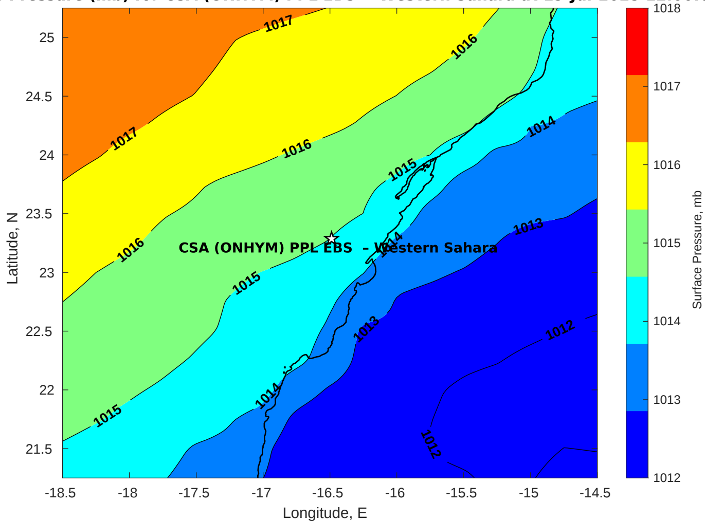
Surface Pressure (mb) for CSA (ONHYM) PPL EBS - Western Sahara at 19-Jul-2025 12:00:00
