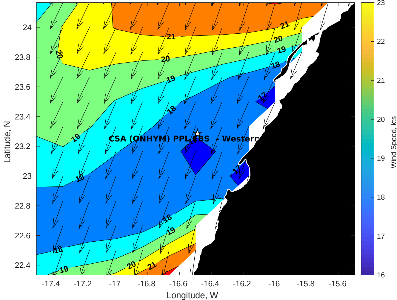
Winds (kts) for CSA (ONHYM) PPL EBS - Western Sahara at 19-Jul-2025 21:00:00
