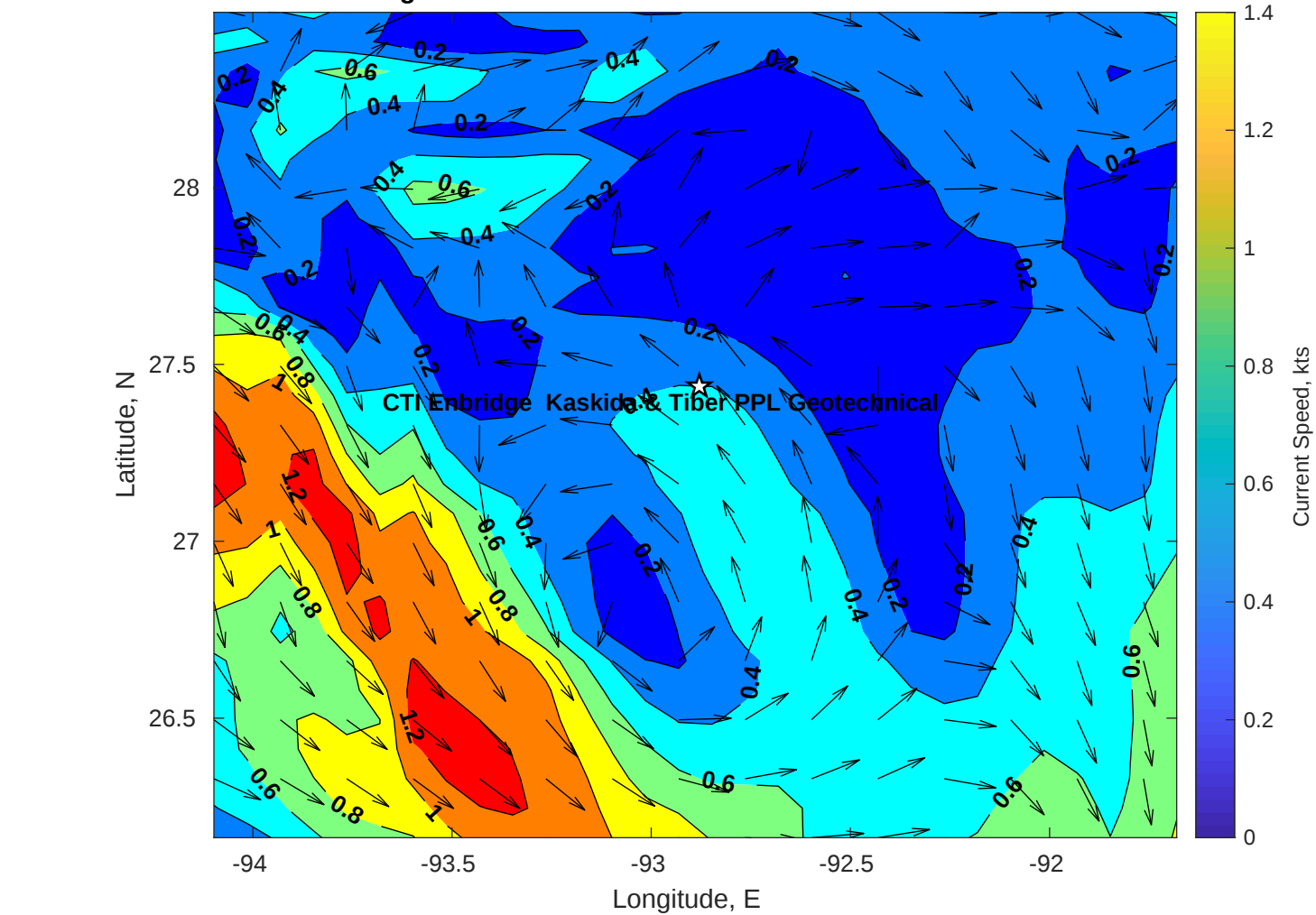
Surface Currents for CTI Enbridge Kaskida & Tiber PPL Geotechnical at 19-Jul-2025 00:00:00
