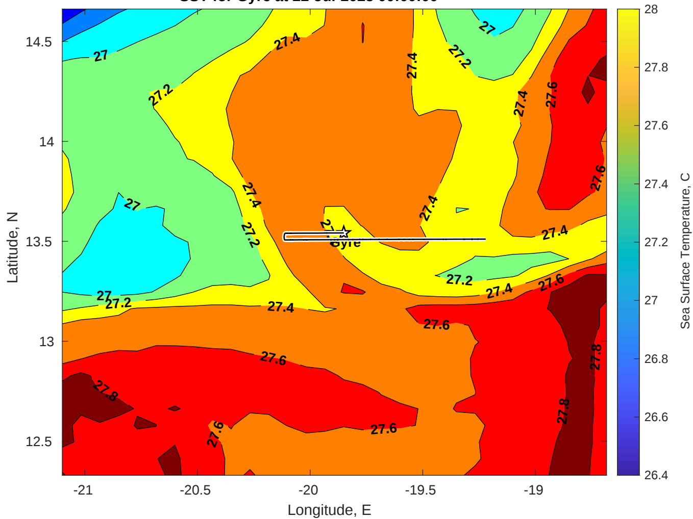
SST for Gyre at 22-Jul-2025 00:00:00
