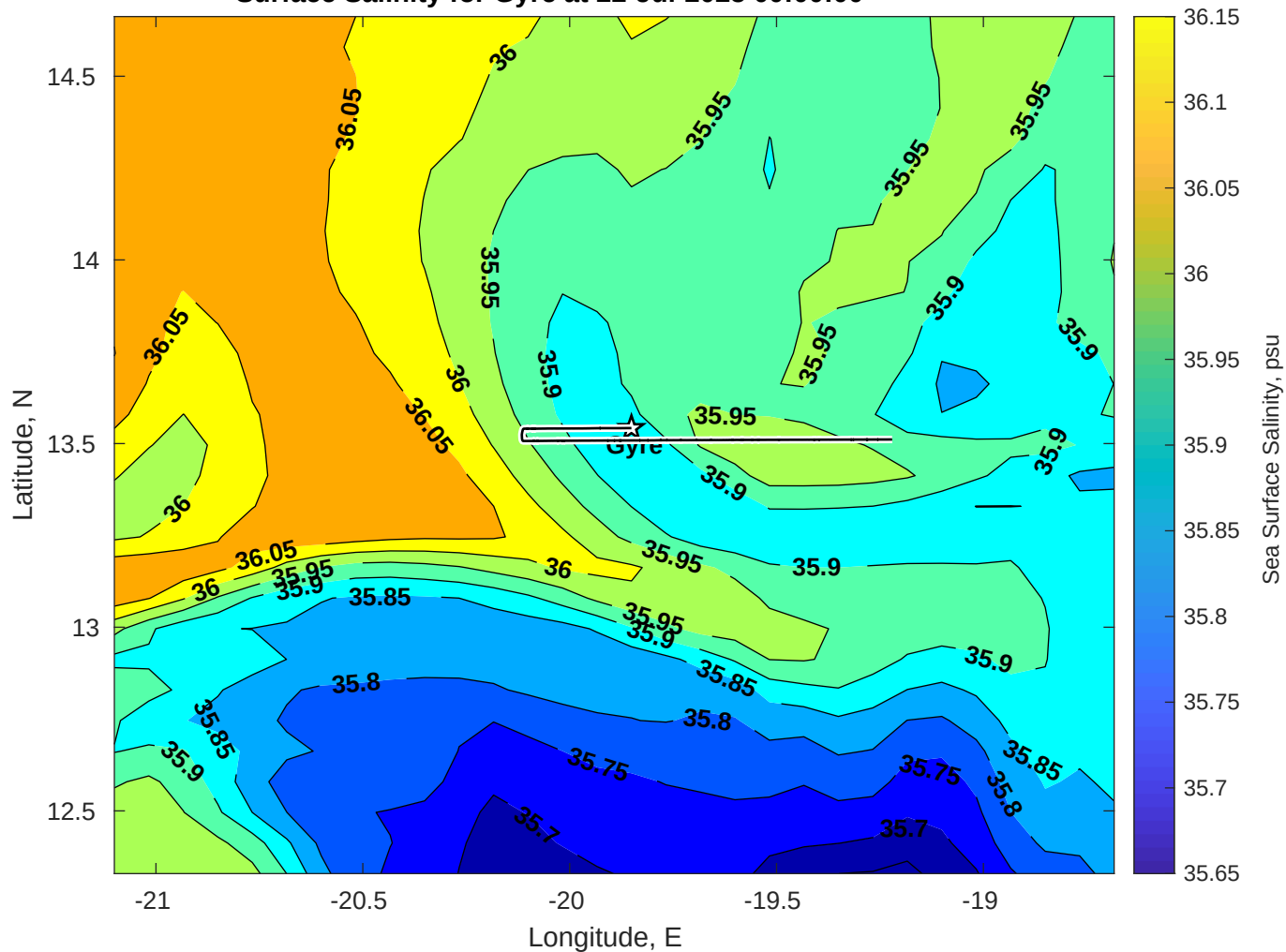
Surface Salinity for Gyre at 22-Jul-2025 00:00:00
