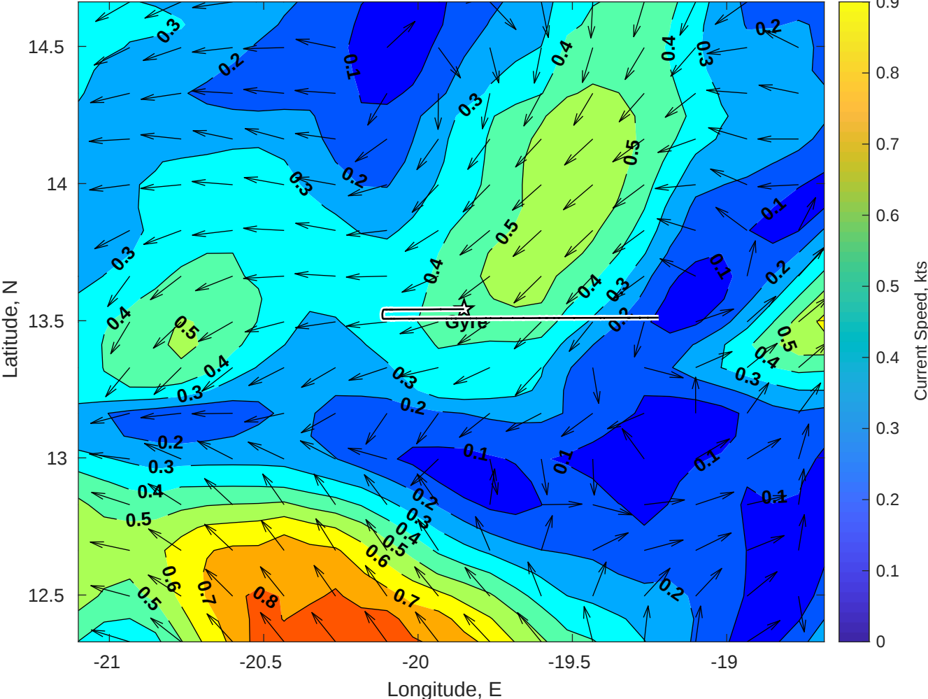
Surface Currents for Gyre at 22-Jul-2025 00:00:00
