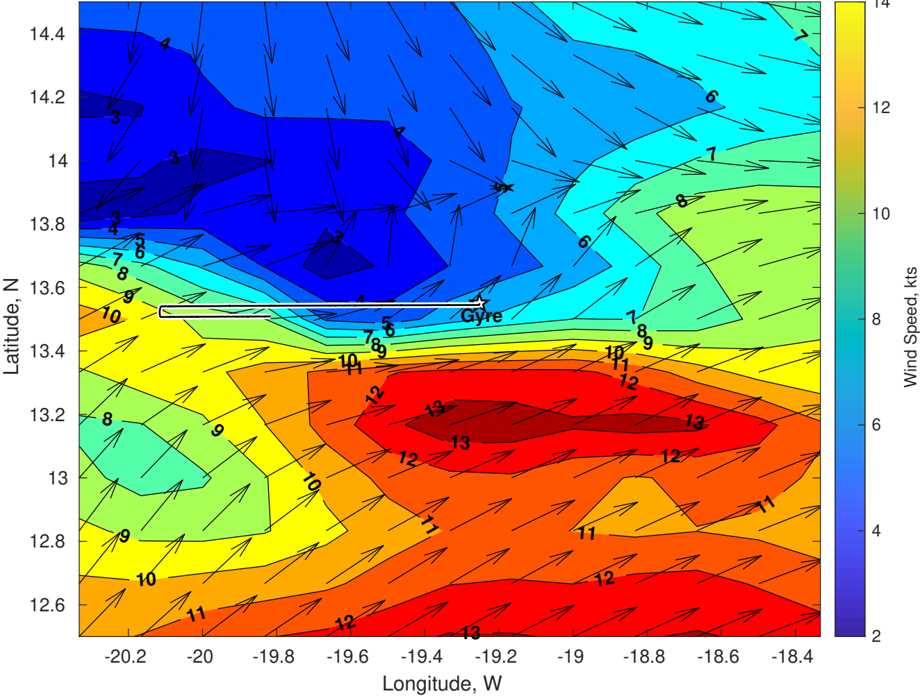
Winds (kts) for Gyre at 23-Jul-2025 09:00:00
