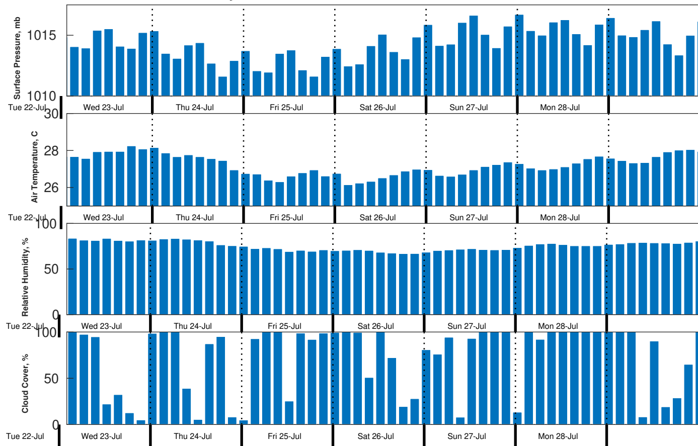
Met Forecast for Gyre from 22-Jul-2025 23:00:00 to 29-Jul-2025 23:00:00
