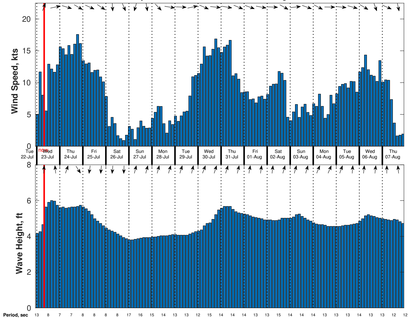
Wind & Wave Forecast for Gyre from 22-Jul-2025 23:00:00 to 07-Aug-2025 23:00:00
