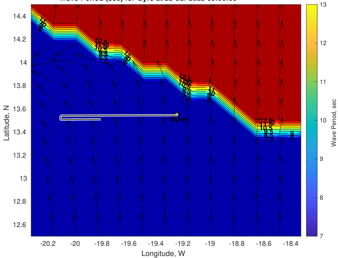
Wave Period (sec) for Gyre at 23-Jul-2025 09:00:00
