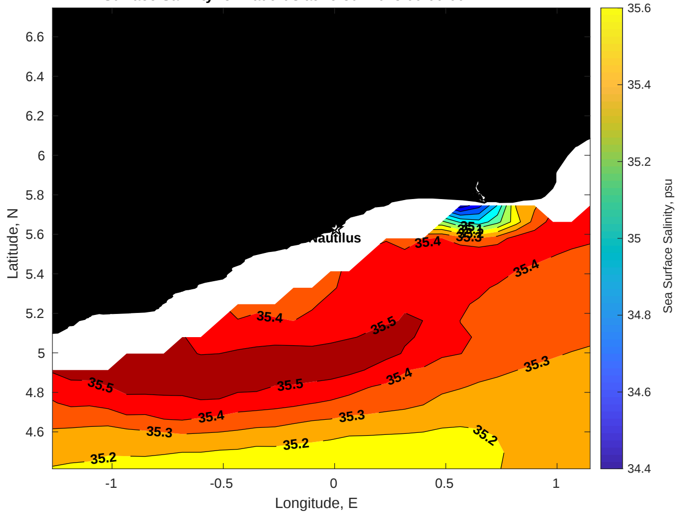
Surface Salinity for Nautilus at 19-Jul-2025 00:00:00
