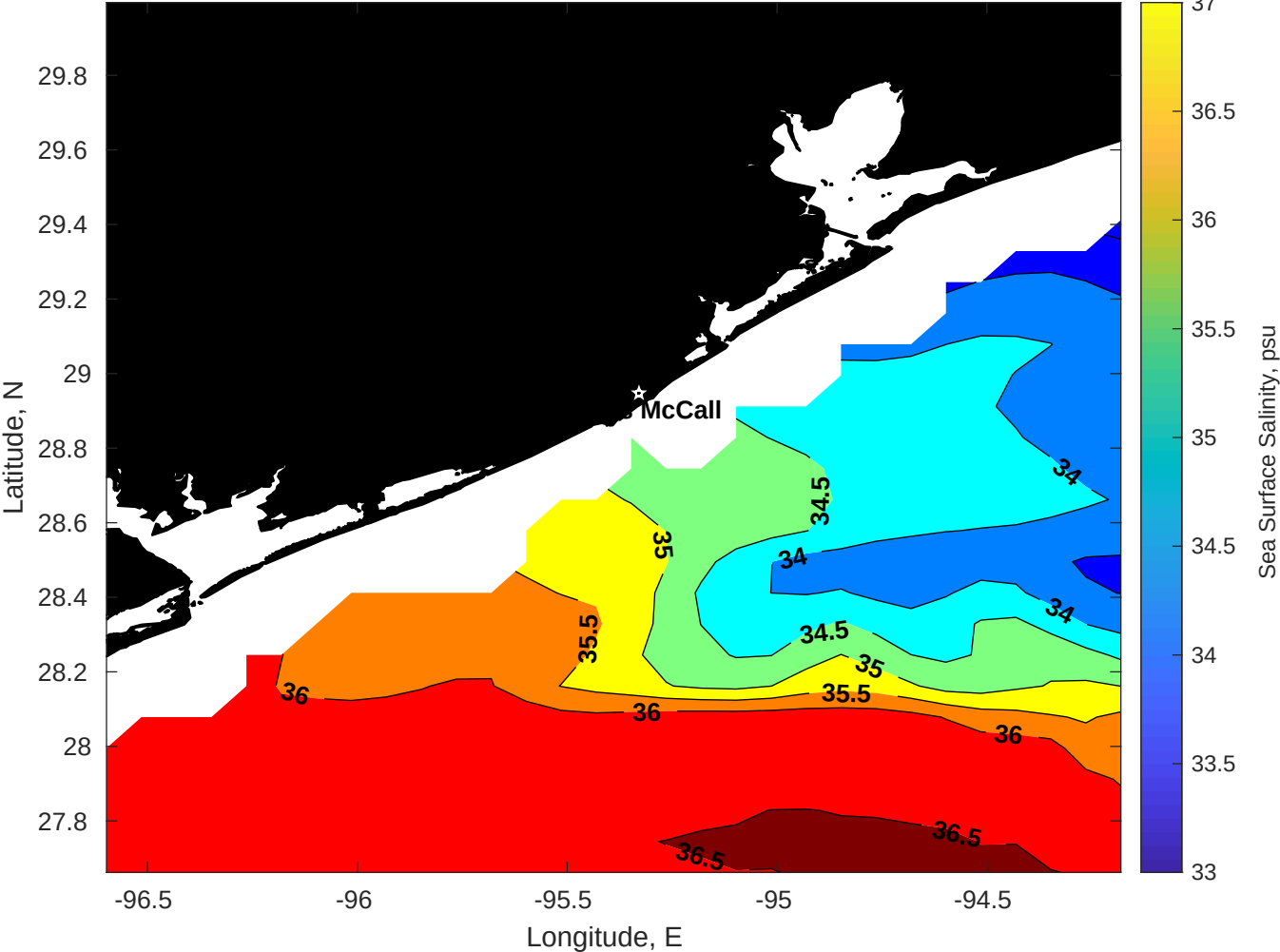
Surface Salinity for Brooks McCall at 23-Jul-2025 00:00:00
