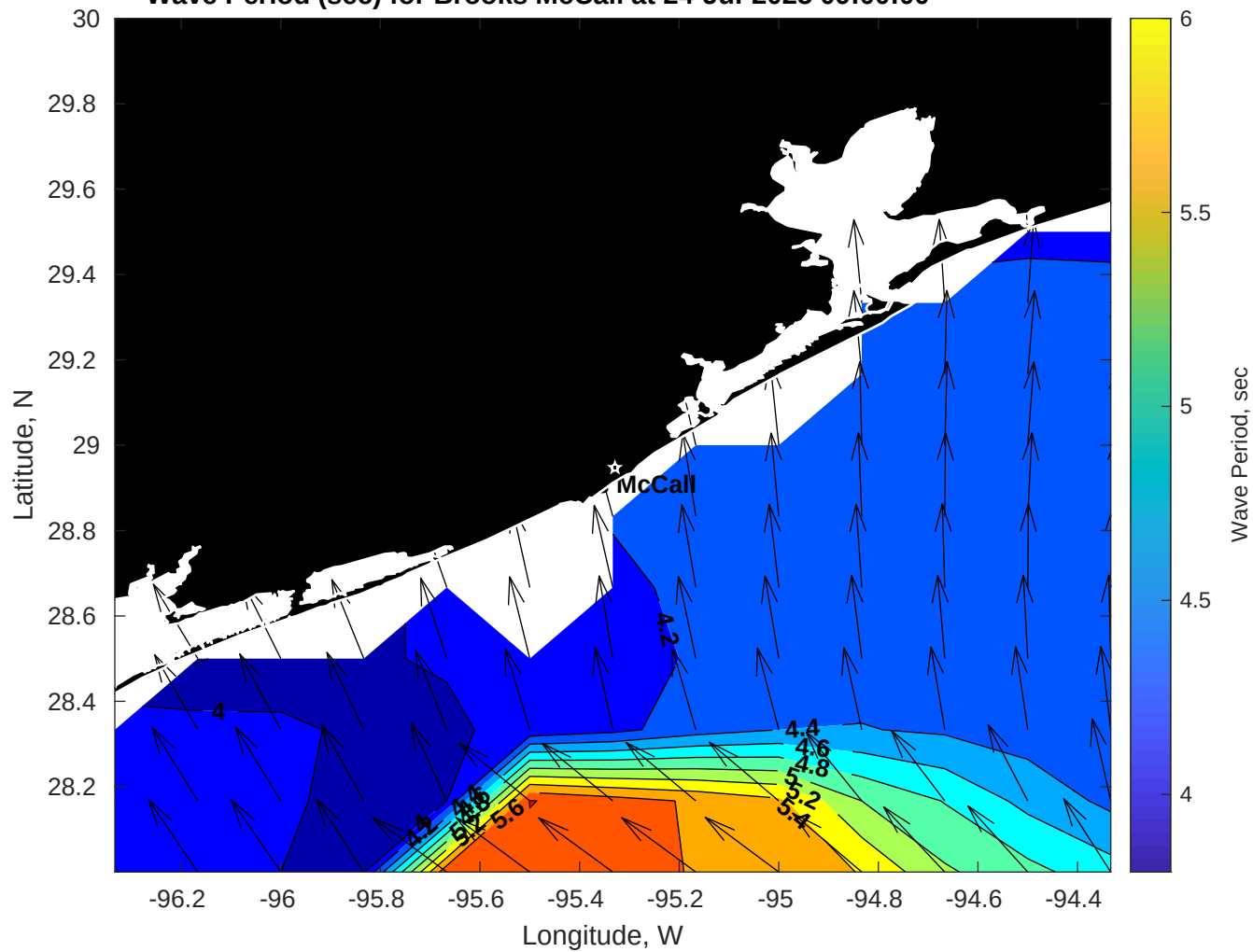
Wave Period (sec) for Brooks McCall at 24-Jul-2025 09:00:00
