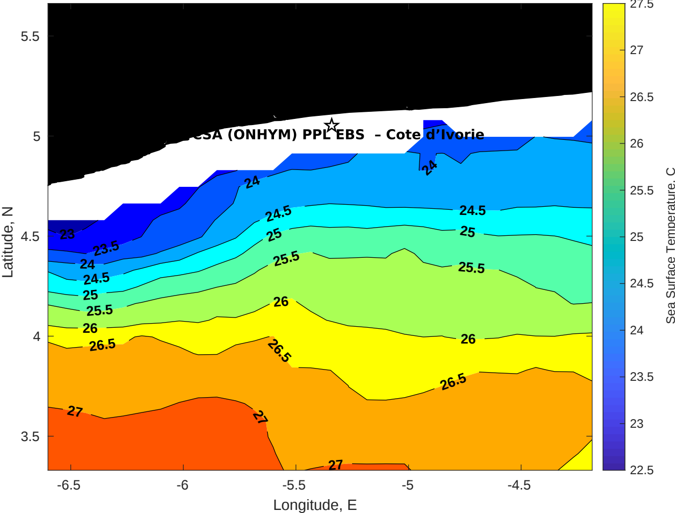
SST for CSA (ONHYM) PPL EBS - Cote d'Ivoire at 19-Jul-2025 00:00:00
