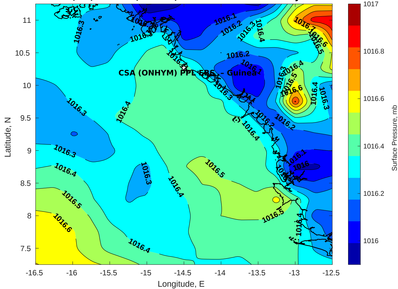
Surface Pressure (mb) for CSA (ONHYM) PPL EBS - Guinea at 19-Jul-2025 12:00:00
