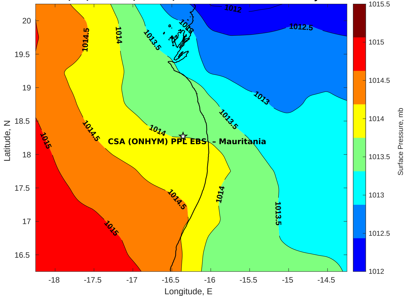
Surface Pressure (mb) for CSA (ONHYM) PPL EBS - Mauritania at 20-Jul-2025 12:00:00
