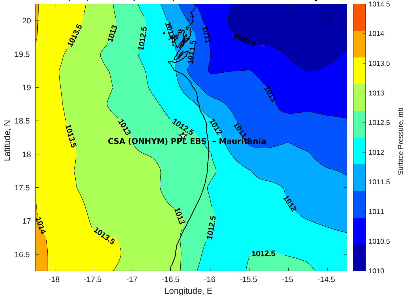
Surface Pressure (mb) for CSA (ONHYM) PPL EBS - Mauritania at 21-Jul-2025 12:00:00
