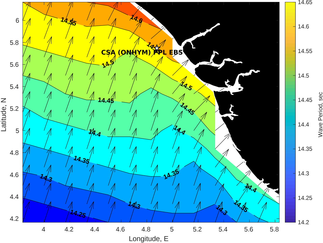
Wave Period (sec) for CSA (ONHYM) PPL EBS - Nigeria at 19-Jul-2025 21:00:00
