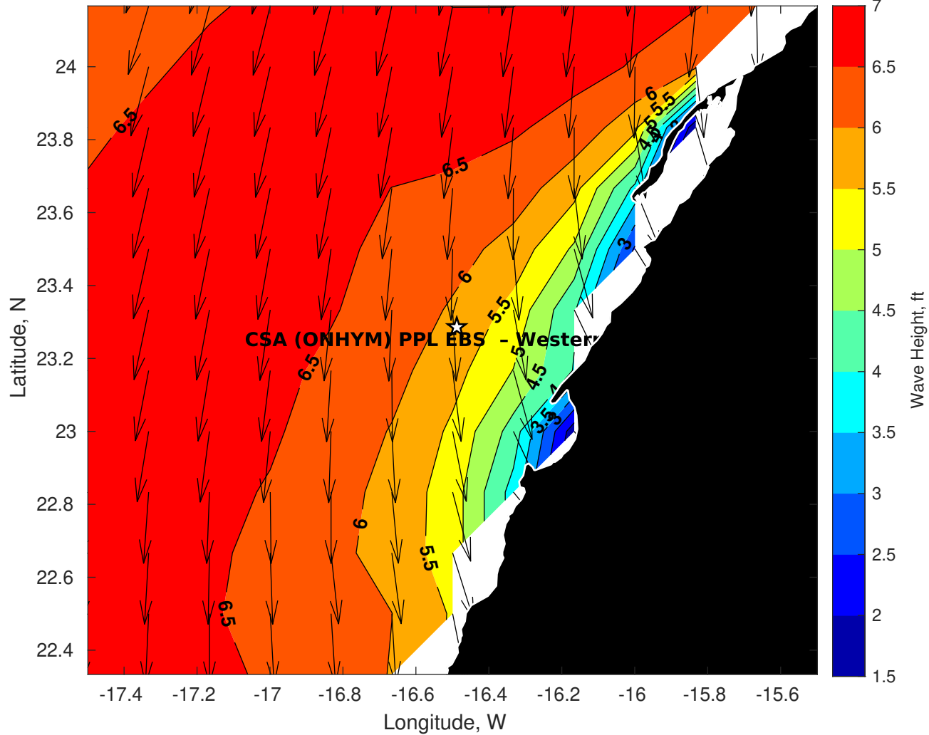
Wave Height (ft) for CSA (ONHYM) PPL EBS - Western Sahara at 19-Jul-2025 21:00:00
