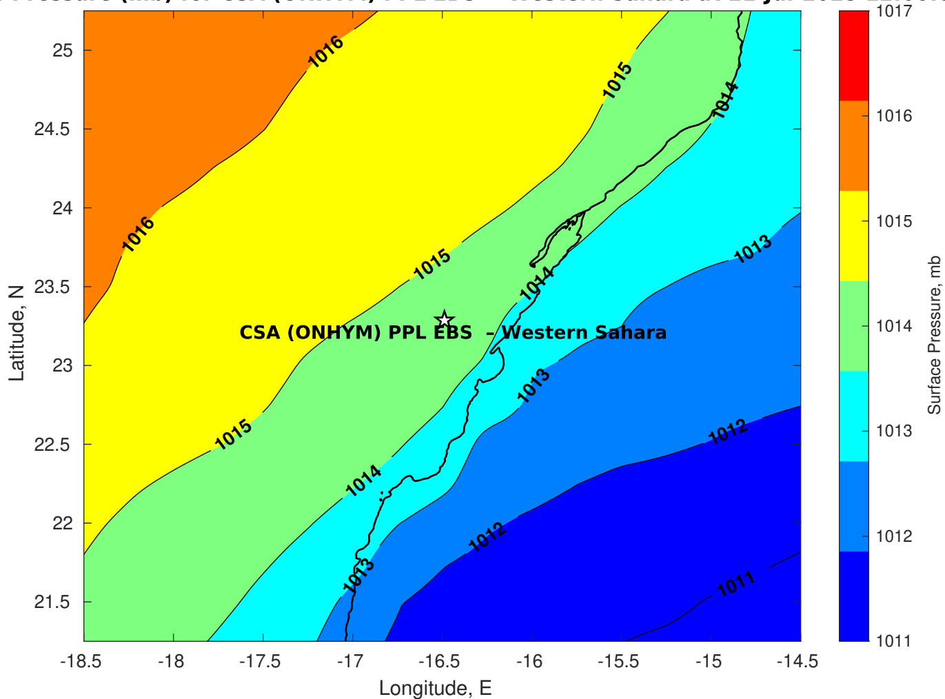
Surface Pressure (mb) for CSA (ONHYM) PPL EBS - Western Sahara at 21-Jul-2025 12:00:00
