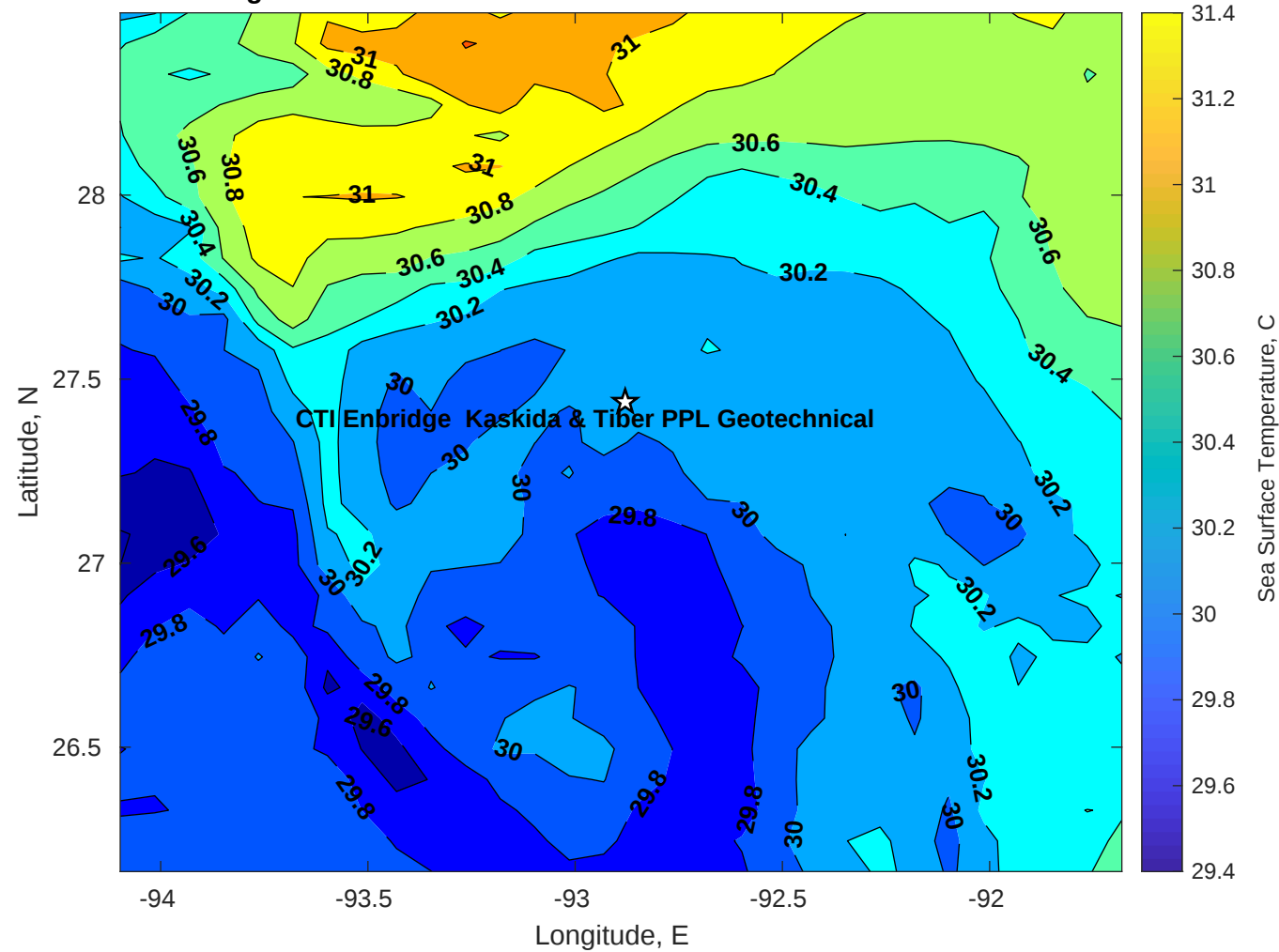
SST for CTI Enbridge Kaskida & Tiber PPL Geotechnical at 19-Jul-2025 00:00:00
