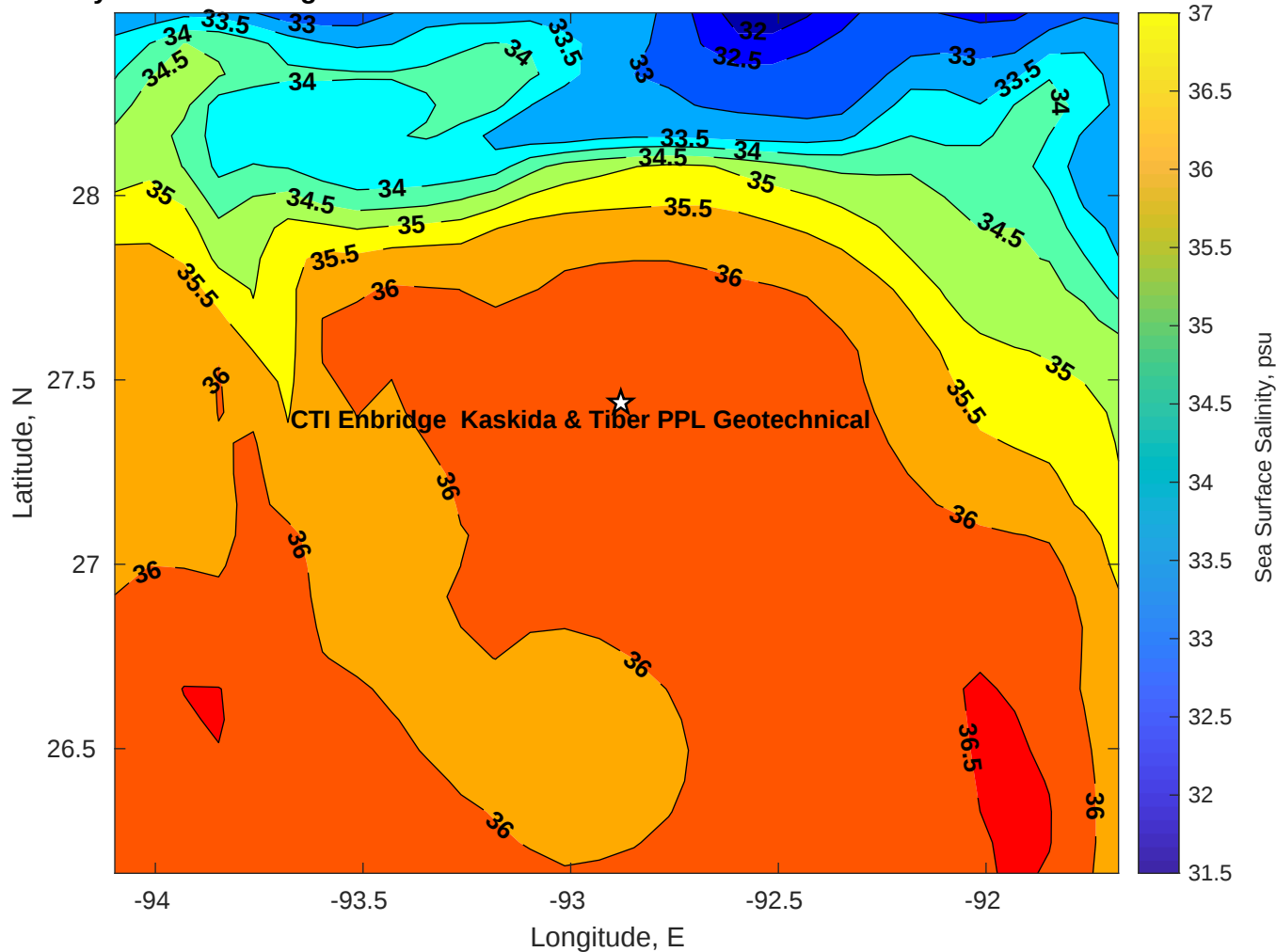
Surface Salinity for CTI Enbridge Kaskida & Tiber PPL Geotechnical at 19-Jul-2025 00:00:00
