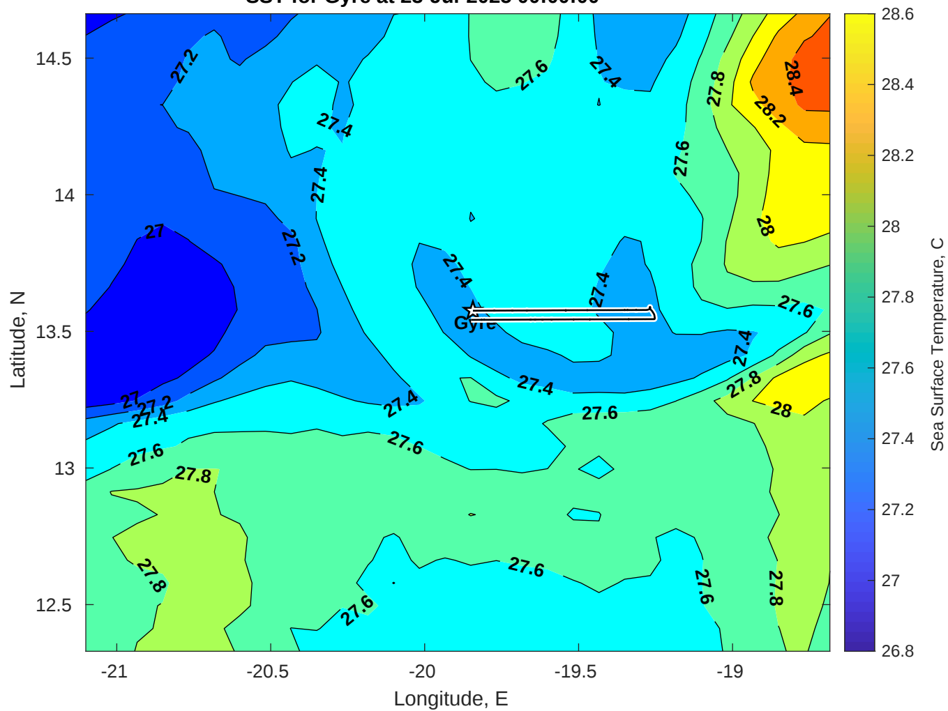
SST for Gyre at 23-Jul-2025 00:00:00
