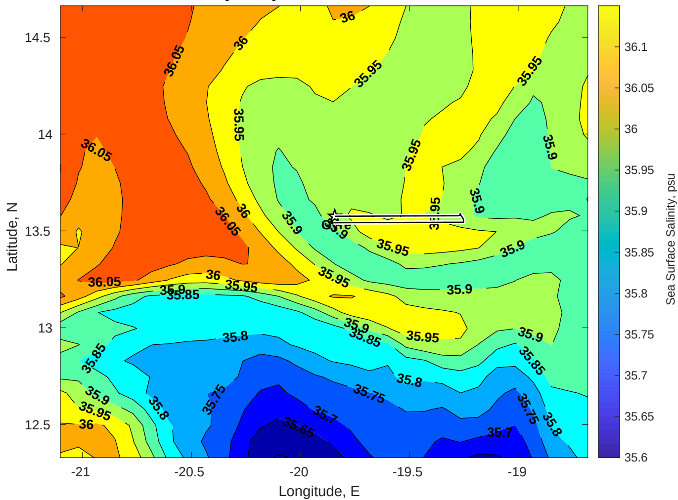
Surface Salinity for Gyre at 23-Jul-2025 00:00:00
