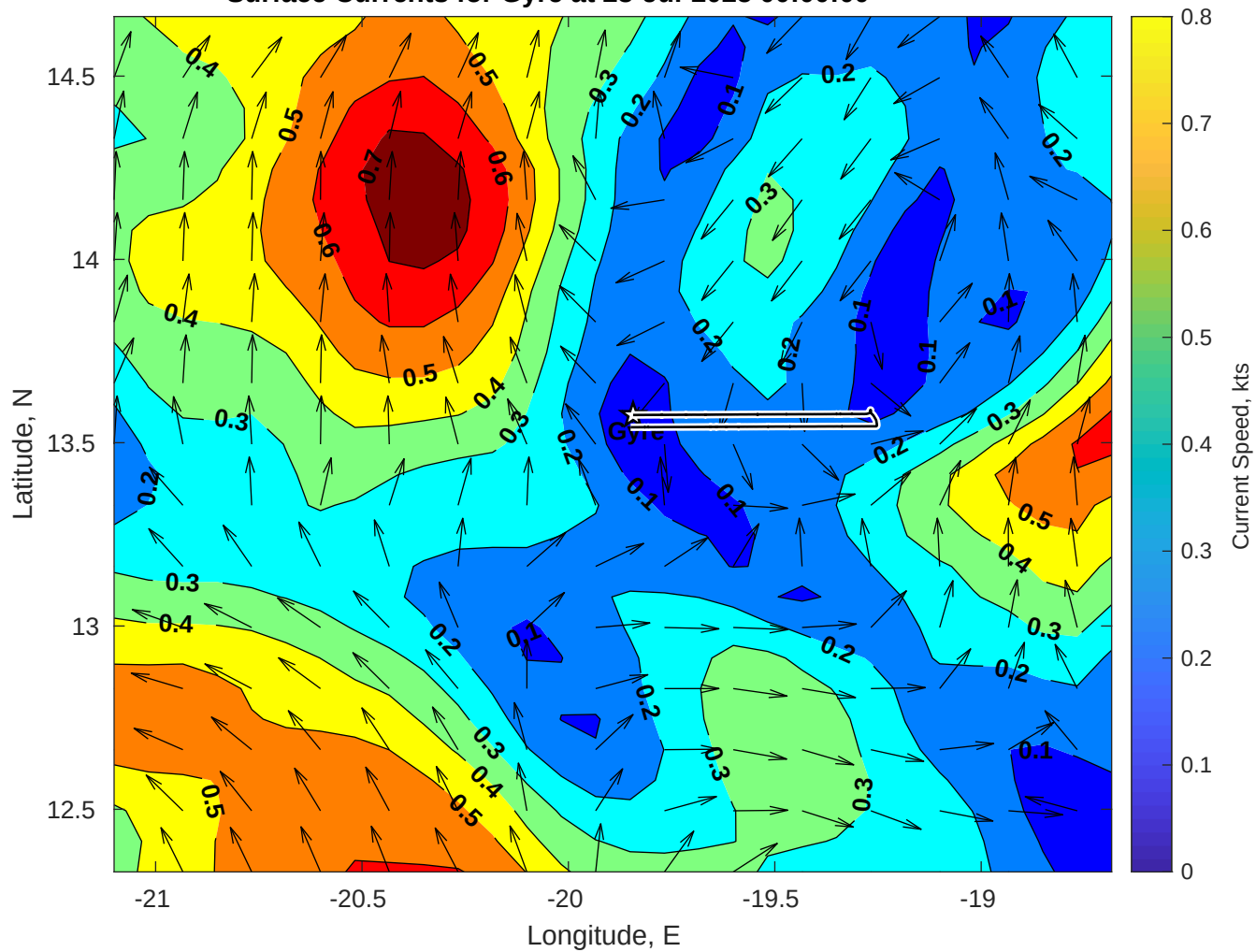
Surface Currents for Gyre at 23-Jul-2025 00:00:00
