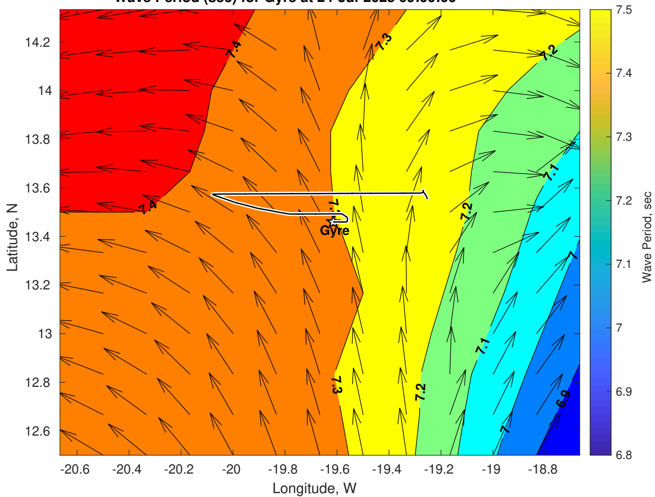
Wave Period (sec) for Gyre at 24-Jul-2025 09:00:00
