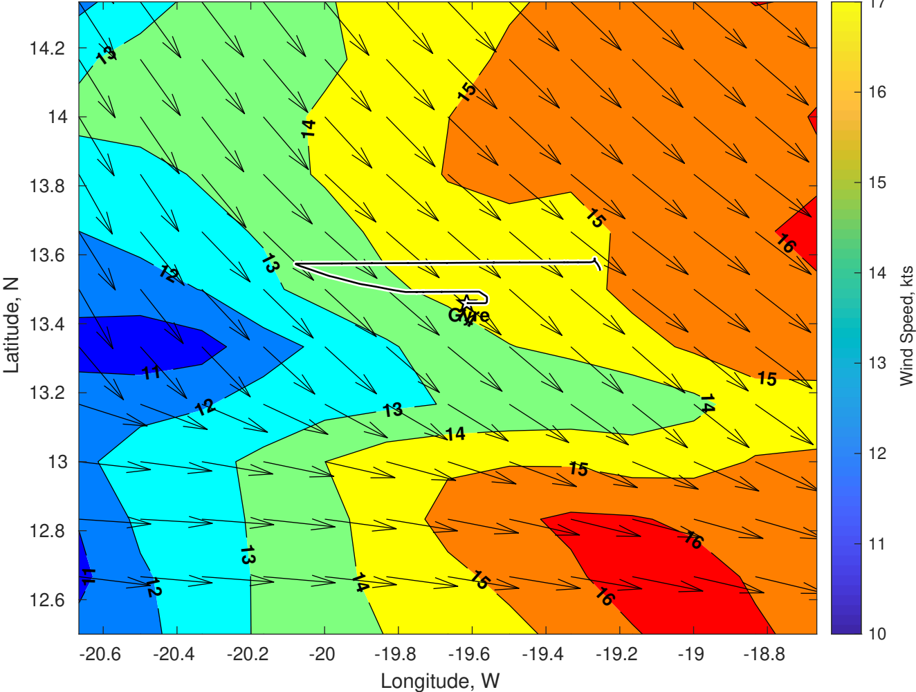
Winds (kts) for Gyre at 24-Jul-2025 09:00:00
