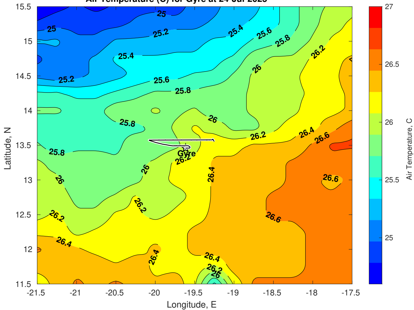
Air Temperature (C) for Gyre at 24-Jul-2025
