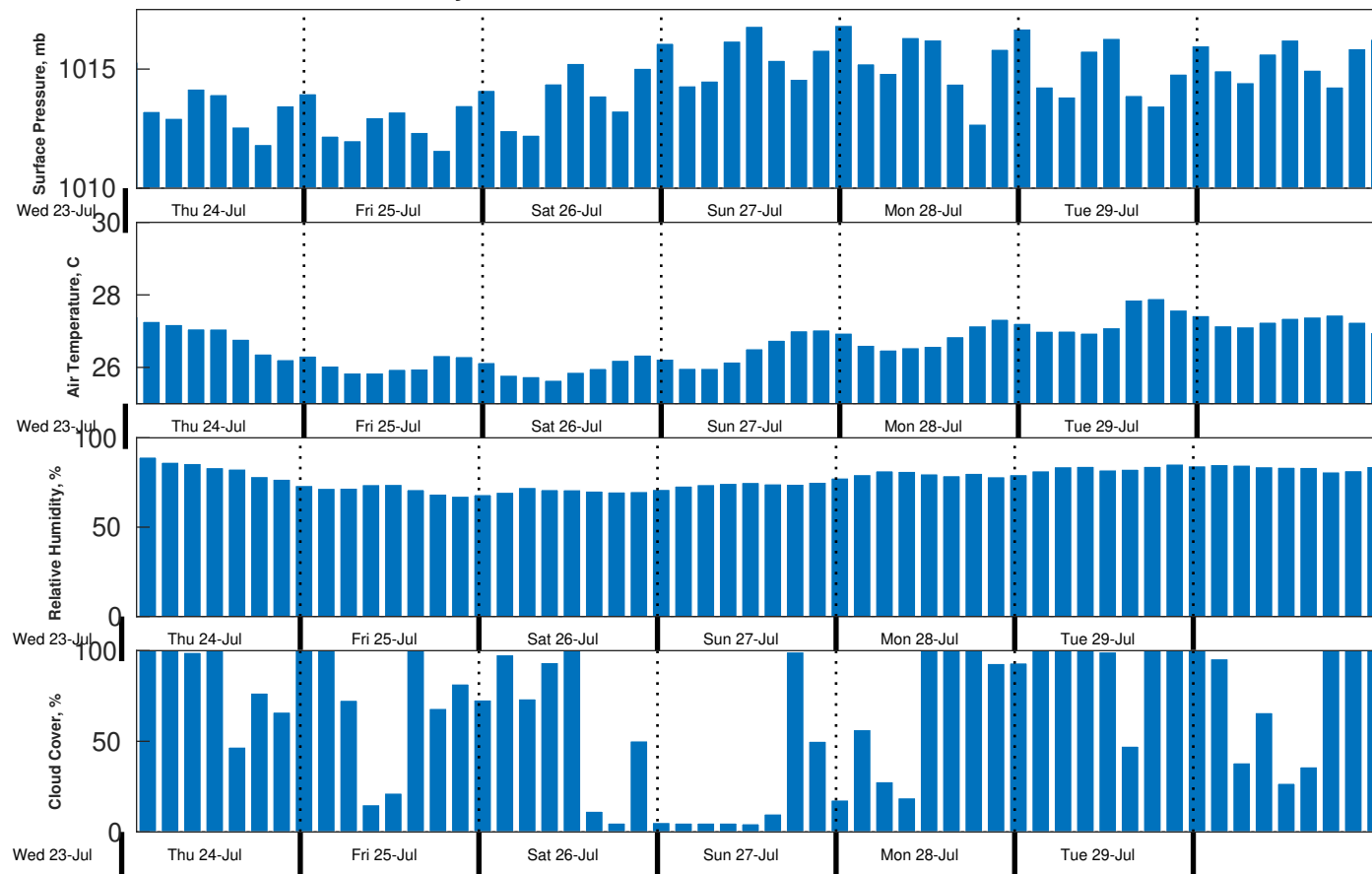
Met Forecast for Gyre from 23-Jul-2025 23:00:00 to 30-Jul-2025 23:00:00
