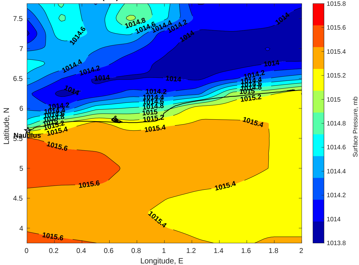
Surface Pressure (mb) for Nautilus at 20-Jul-2025 12:00:00
