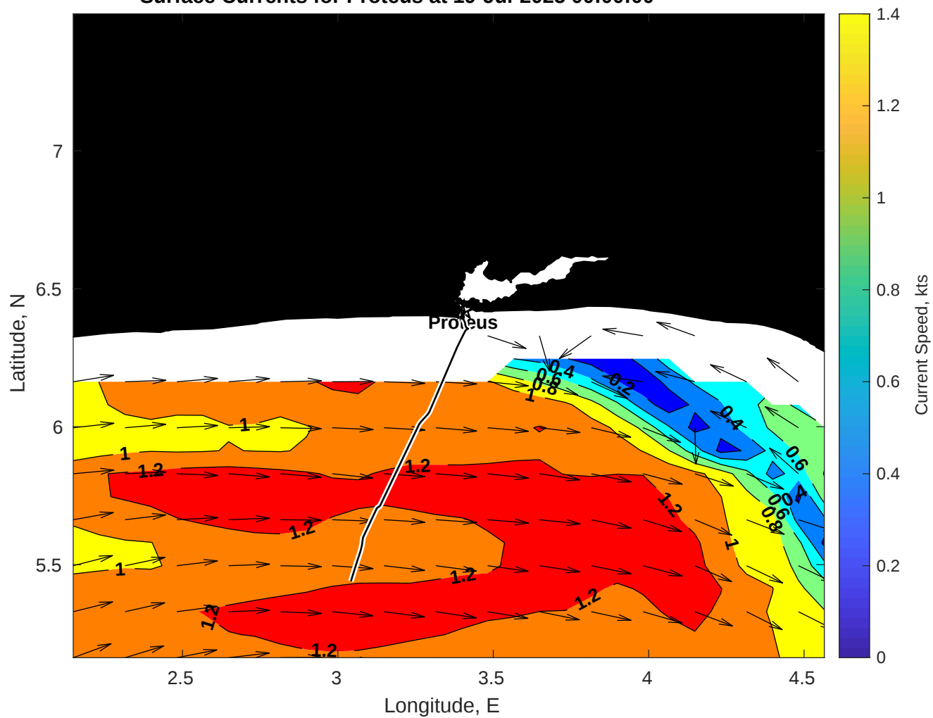
Surface Currents for Proteus at 19-Jul-2025 00:00:00
