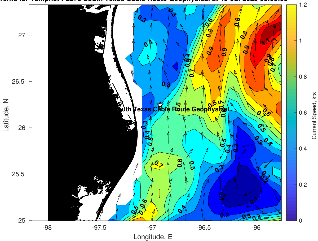
Surface Currents for Tampnet P2378 South Texas Cable Route Geophysical at 19-Jul-2025 00:00:00
