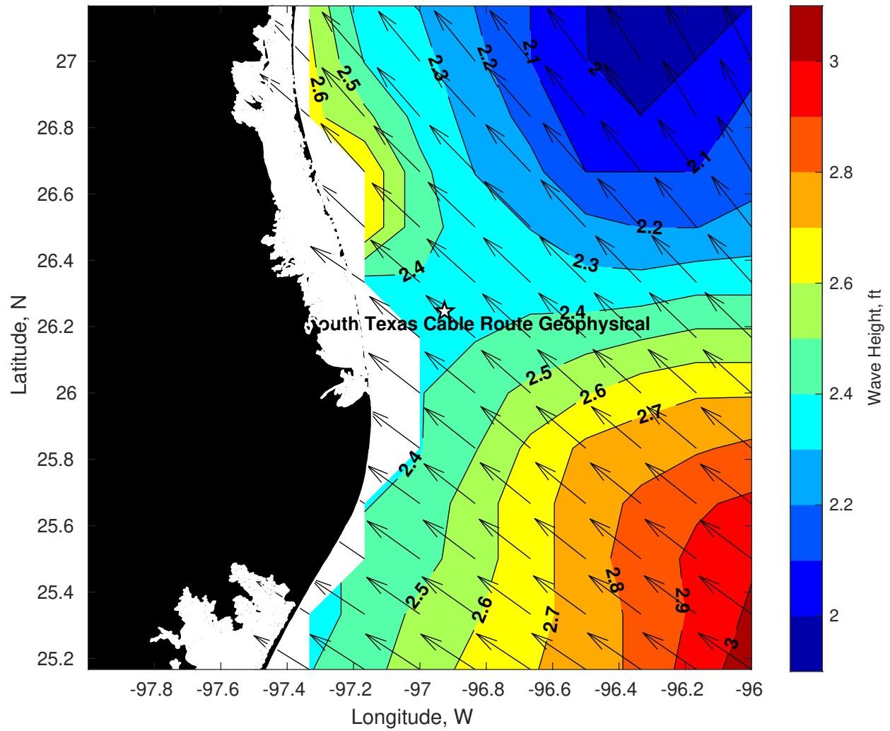
Wave Height (ft) for Tampnet P2378 South Texas Cable Route Geophysical at 19-Jul-2025 21:00:00
