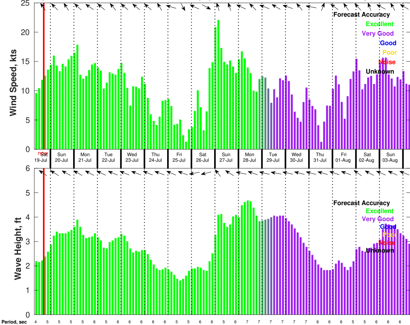
Wind & Wave Forecast for Tampnet P2378 South Texas Cable Route Geophysical from 19-Jul-2025 08:00:00 to 04-Aug-2025 08:00:00
