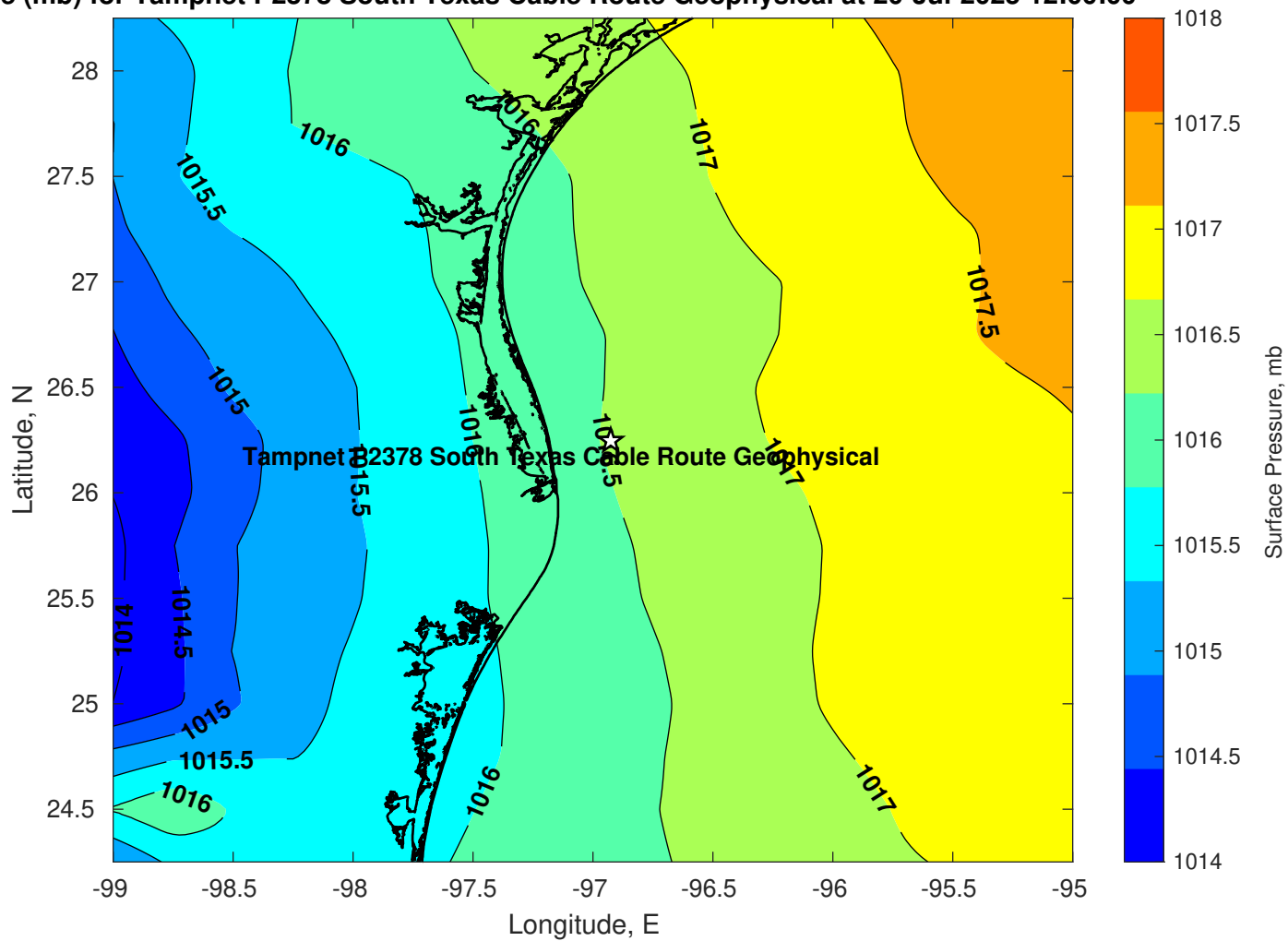
Pressure (mb) for Tampnet P2378 South Texas Cable Route Geophysical at 20-Jul-2025 12:00:00
