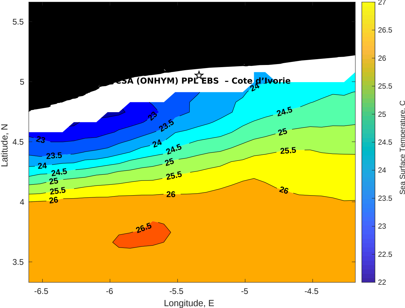
SST for CSA (ONHYM) PPL EBS - Cote d'Ivoire at 24-Jul-2025 00:00:00
