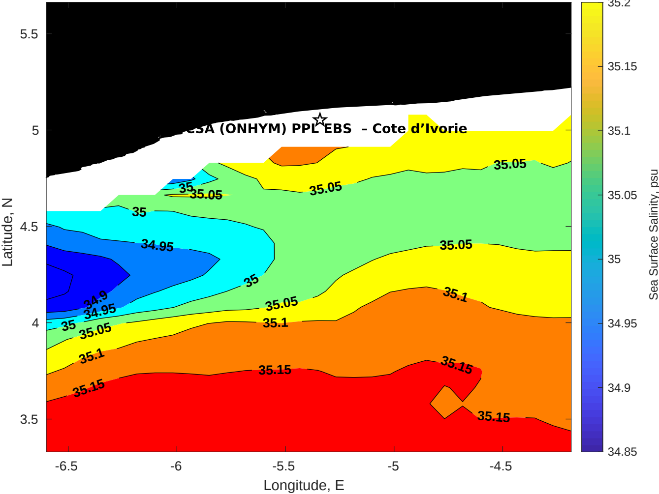
Surface Salinity for CSA (ONHYM) PPL EBS - Cote d'Ivoire at 24-Jul-2025 00:00:00
