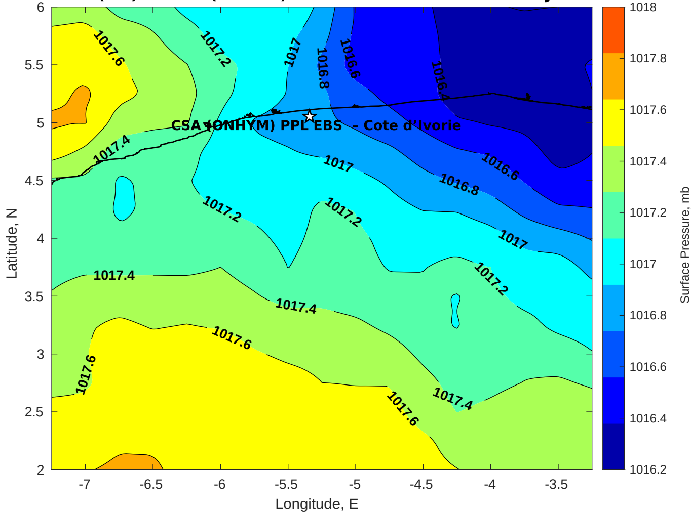
Surface Pressure (mb) for CSA (ONHYM) PPL EBS - Cote d'Ivoire at 27-Jul-2025 00:00:00
