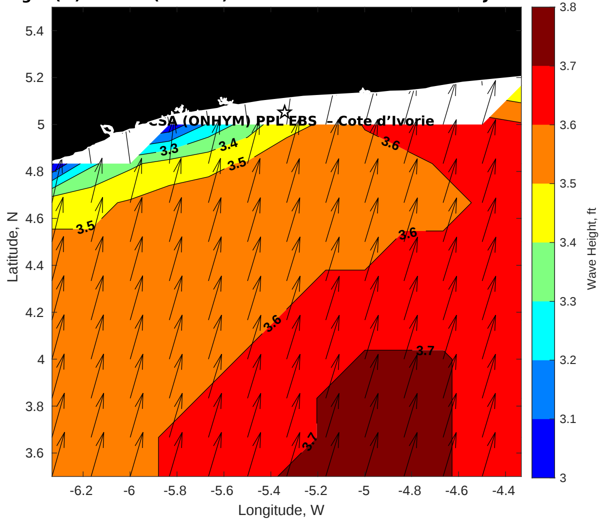
Wave Height (ft) for CSA (ONHYM) PPL EBS - Cote d'Ivoire at 25-Jul-2025 09:00:00
