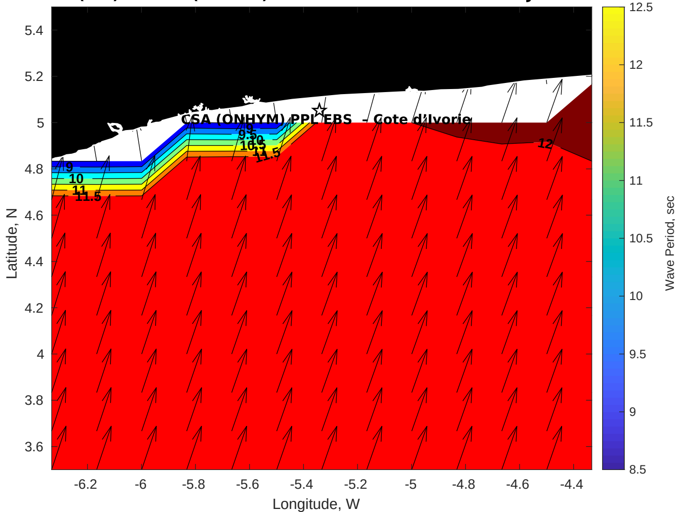
Wave Period (sec) for CSA (ONHYM) PPL EBS - Cote d'Ivoire at 25-Jul-2025 09:00:00
