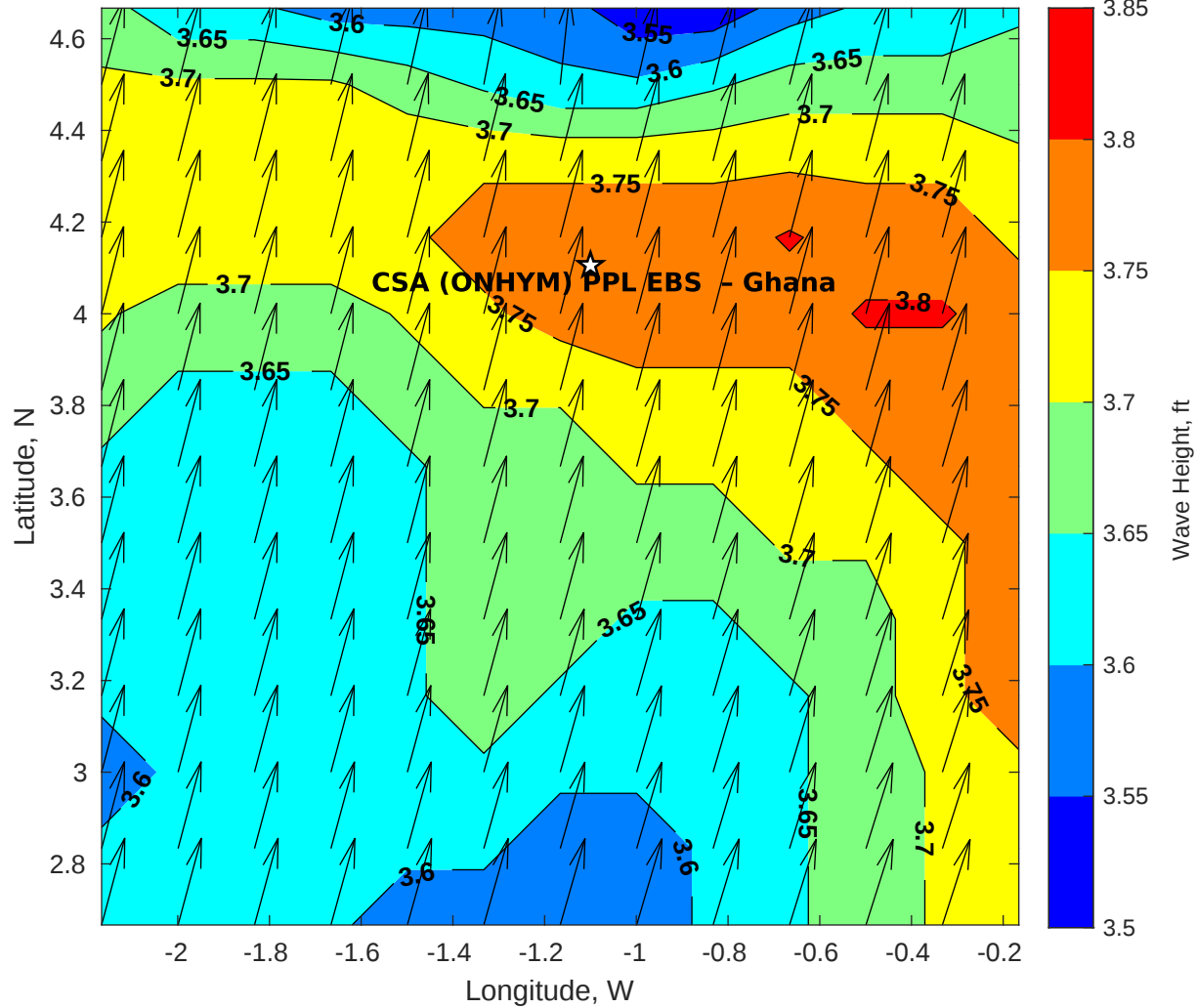
Wave Height (ft) for CSA (ONHYM) PPL EBS - Ghana at 25-Jul-2025 09:00:00
