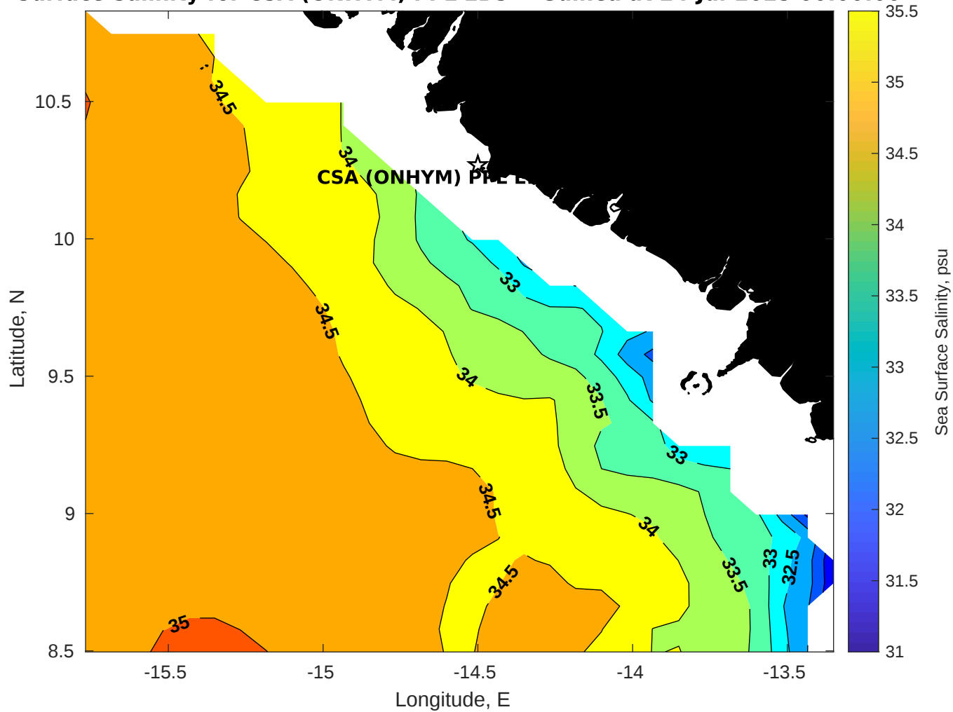
Surface Salinity for CSA (ONHYM) PPL EBS - Guinea at 24-Jul-2025 00:00:00
