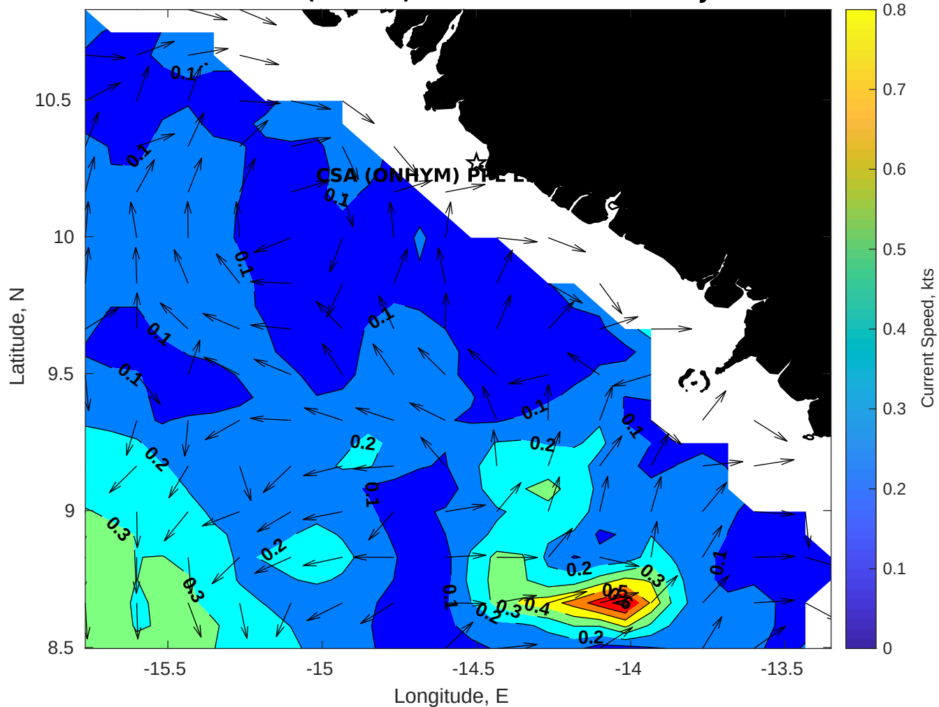
Surface Currents for CSA (ONHYM) PPL EBS - Guinea at 24-Jul-2025 00:00:00
