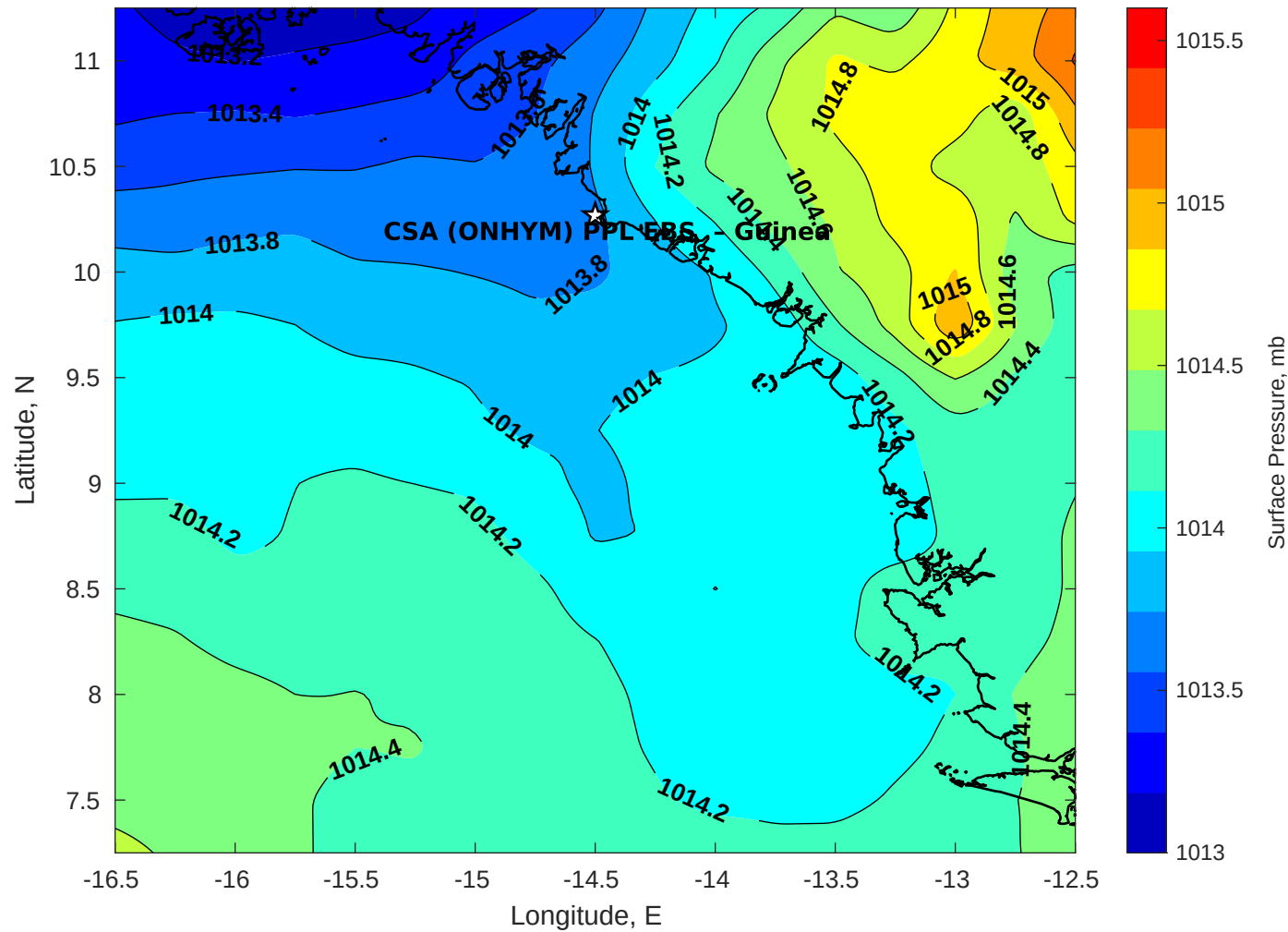
Surface Pressure (mb) for CSA (ONHYM) PPL EBS - Guinea at 25-Jul-2025 00:00:00
