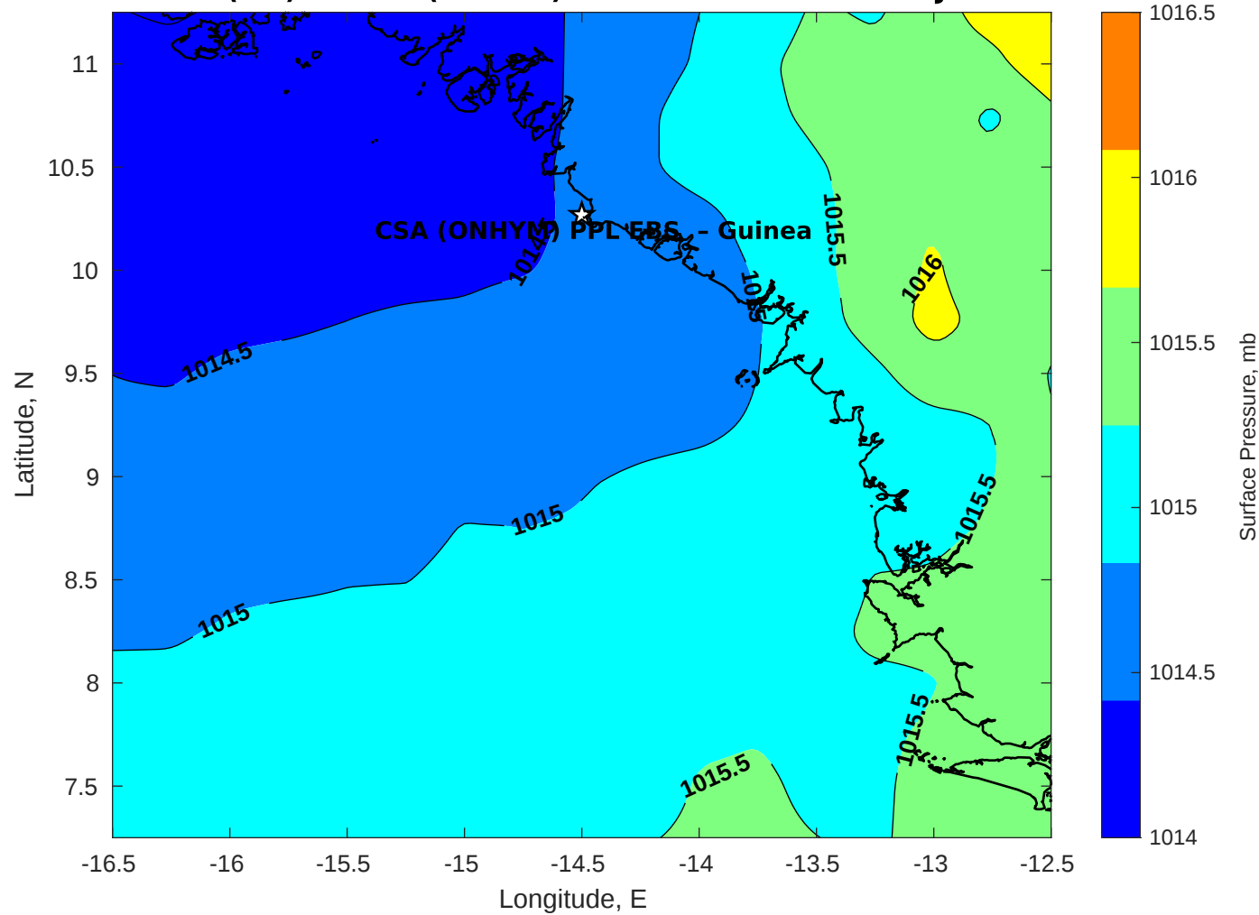
Surface Pressure (mb) for CSA (ONHYM) PPL EBS - Guinea at 26-Jul-2025 00:00:00
