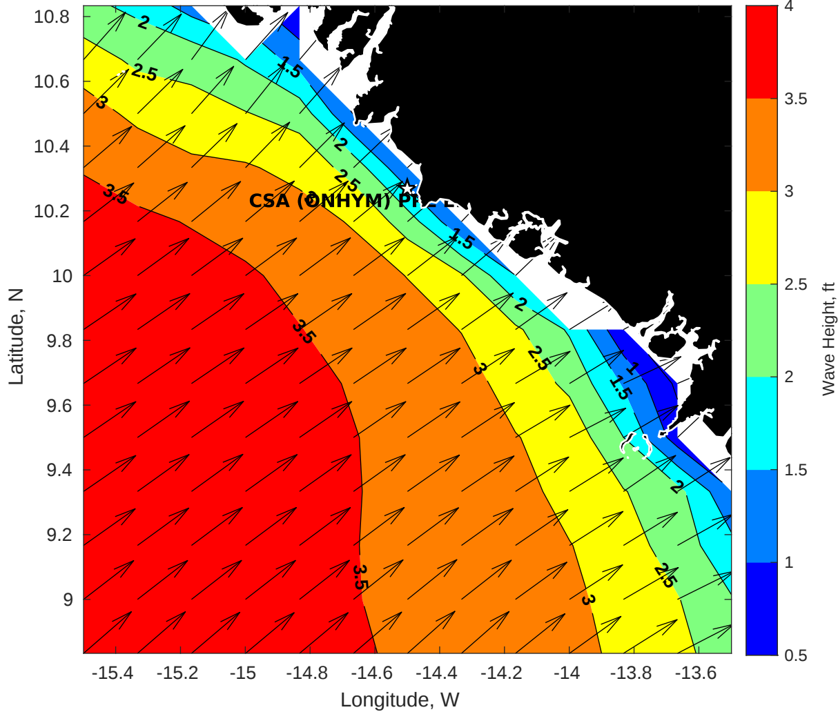
Wave Height (ft) for CSA (ONHYM) PPL EBS - Guinea at 25-Jul-2025 09:00:00
