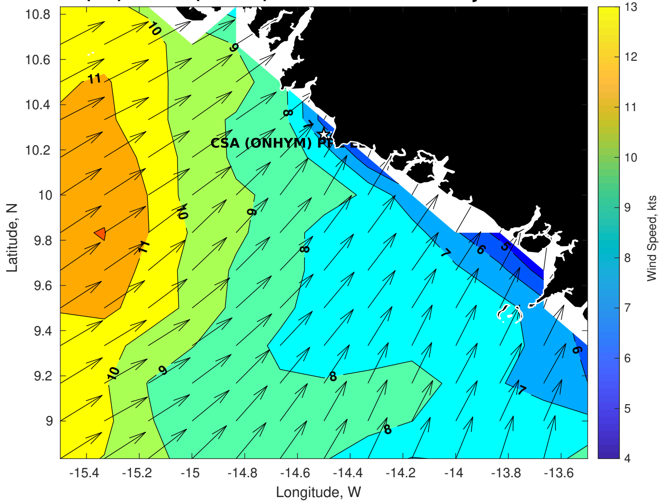
Winds (kts) for CSA (ONHYM) PPL EBS - Guinea at 25-Jul-2025 09:00:00
