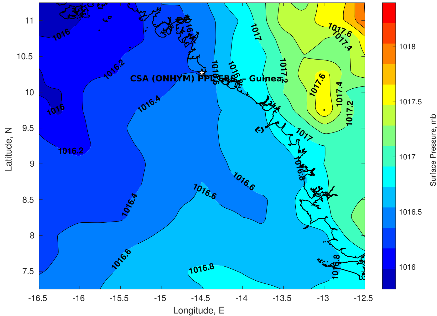
Surface Pressure (mb) for CSA (ONHYM) PPL EBS - Guinea at 27-Jul-2025 00:00:00
