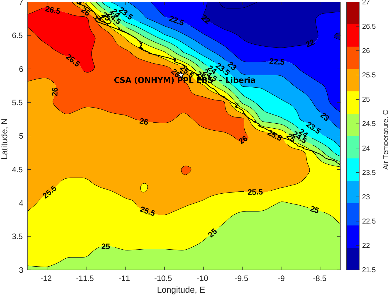
Air Temperature (C) for CSA (ONHYM) PPL EBS - Liberia at 25-Jul-2025
