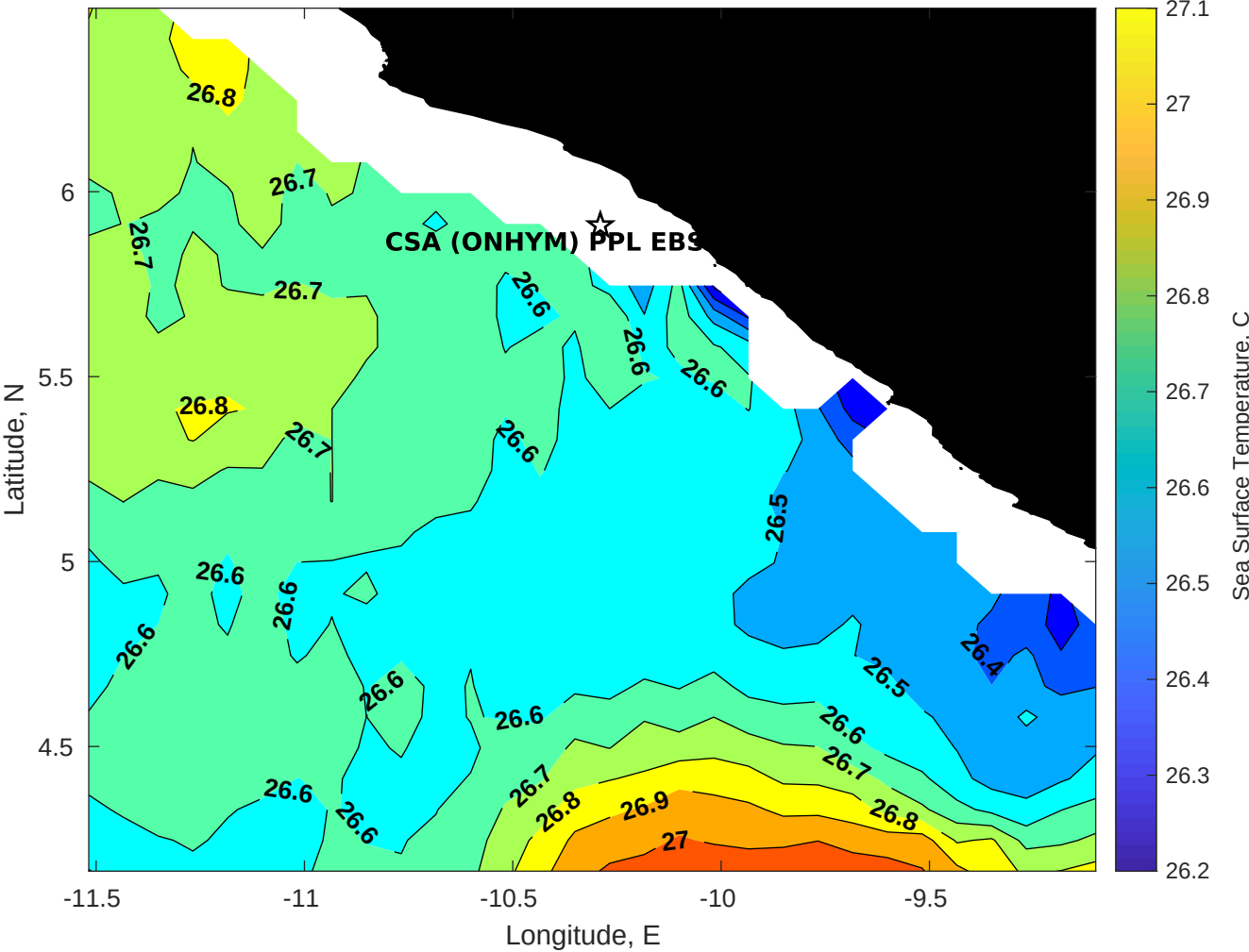
SST for CSA (ONHYM) PPL EBS - Liberia at 24-Jul-2025 00:00:00
