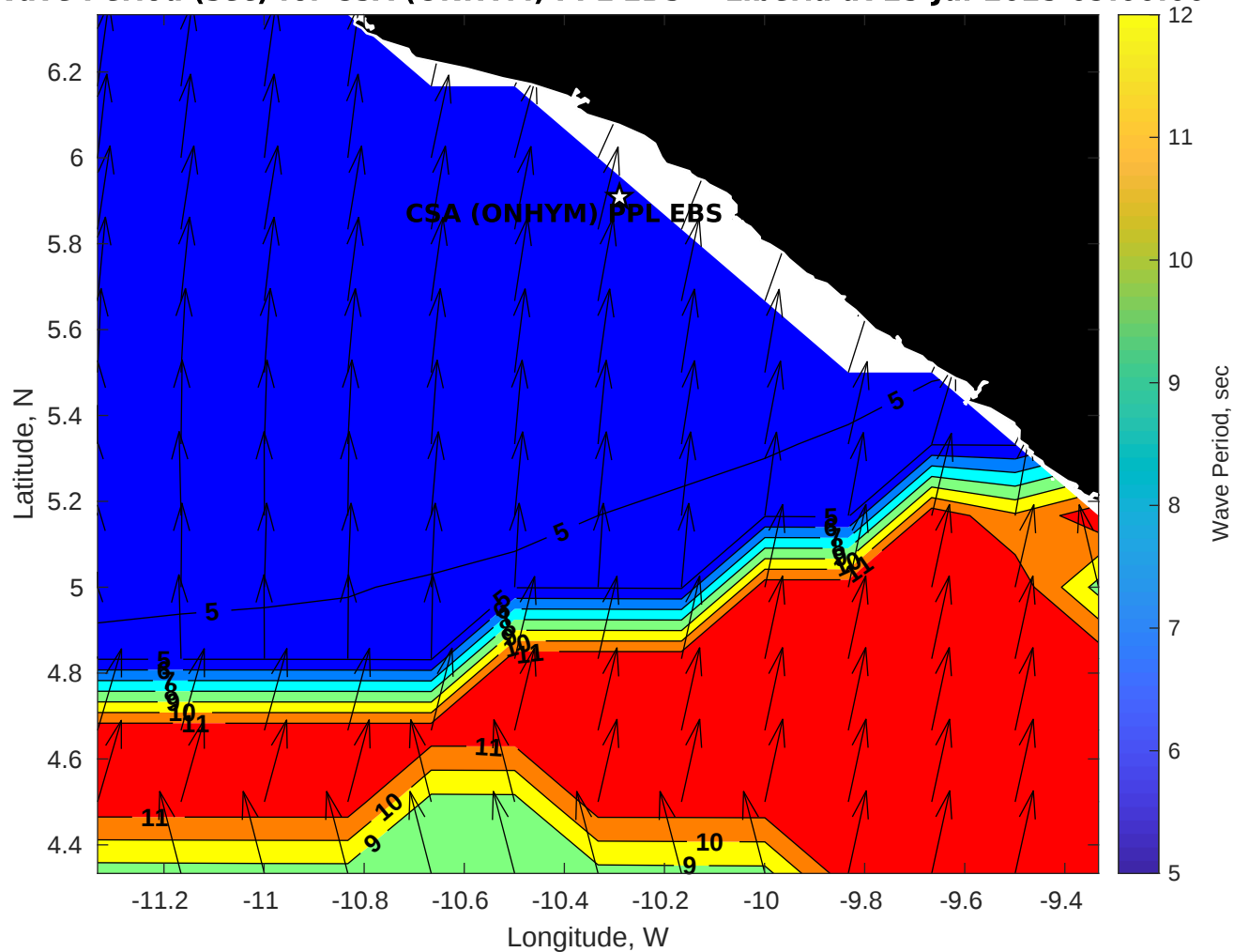
Wave Period (sec) for CSA (ONHYM) PPL EBS - Liberia at 25-Jul-2025 09:00:00
