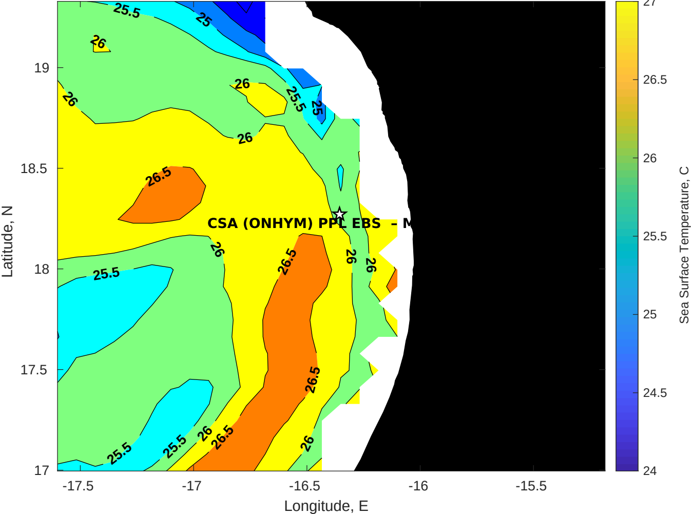
SST for CSA (ONHYM) PPL EBS - Mauritania at 24-Jul-2025 00:00:00
