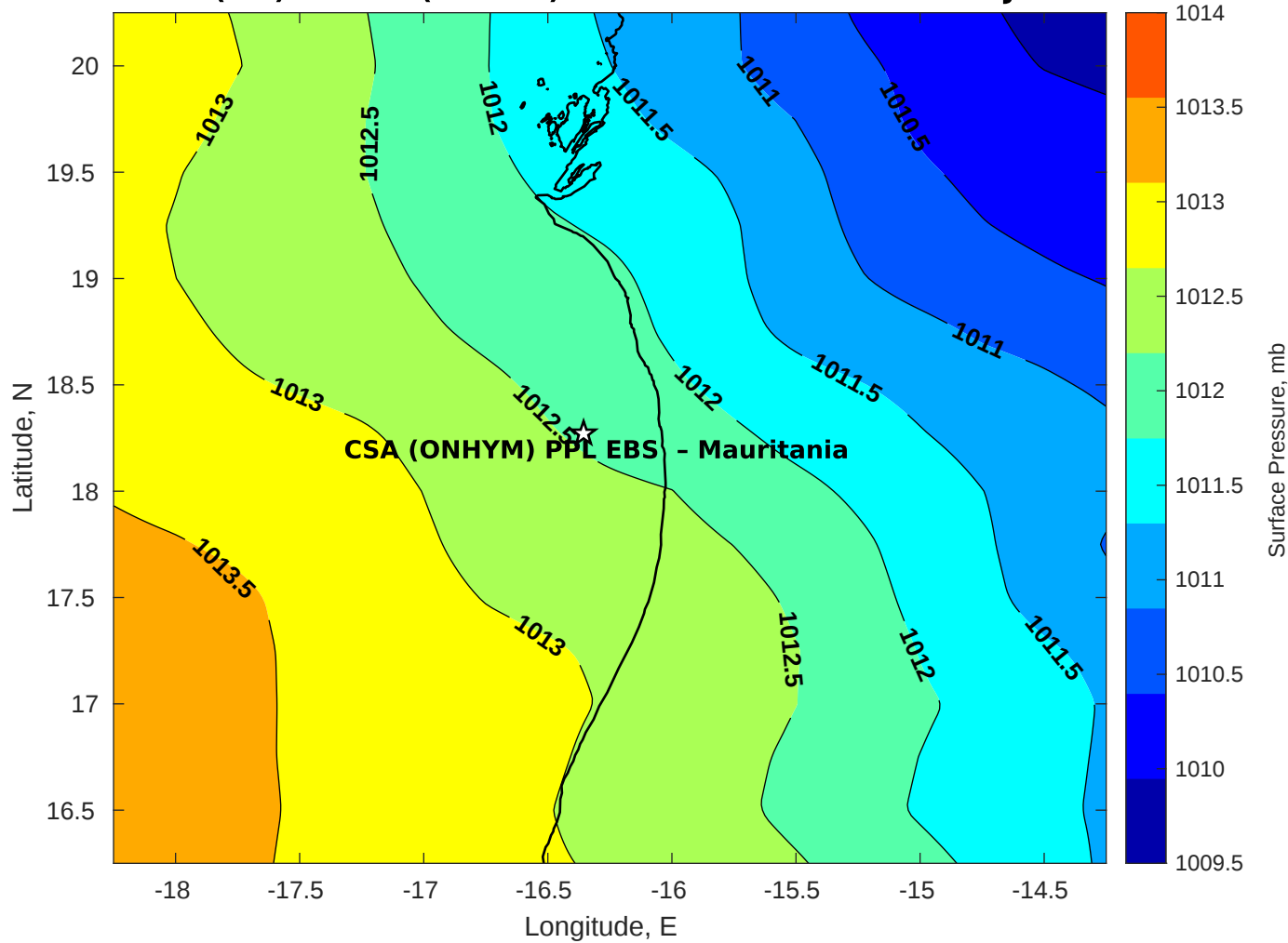
Surface Pressure (mb) for CSA (ONHYM) PPL EBS - Mauritania at 26-Jul-2025 00:00:00
