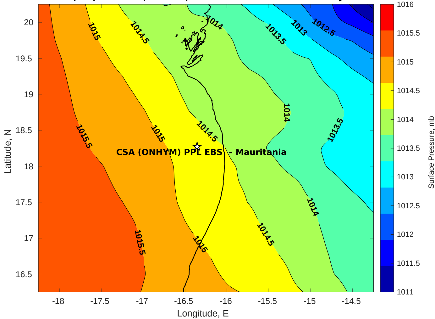
Surface Pressure (mb) for CSA (ONHYM) PPL EBS - Mauritania at 27-Jul-2025 00:00:00
