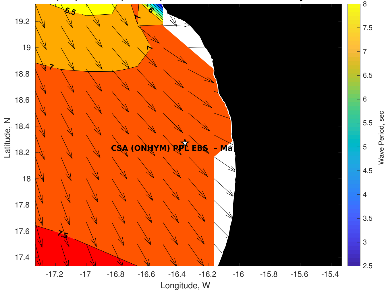
Wave Period (sec) for CSA (ONHYM) PPL EBS - Mauritania at 25-Jul-2025 09:00:00
