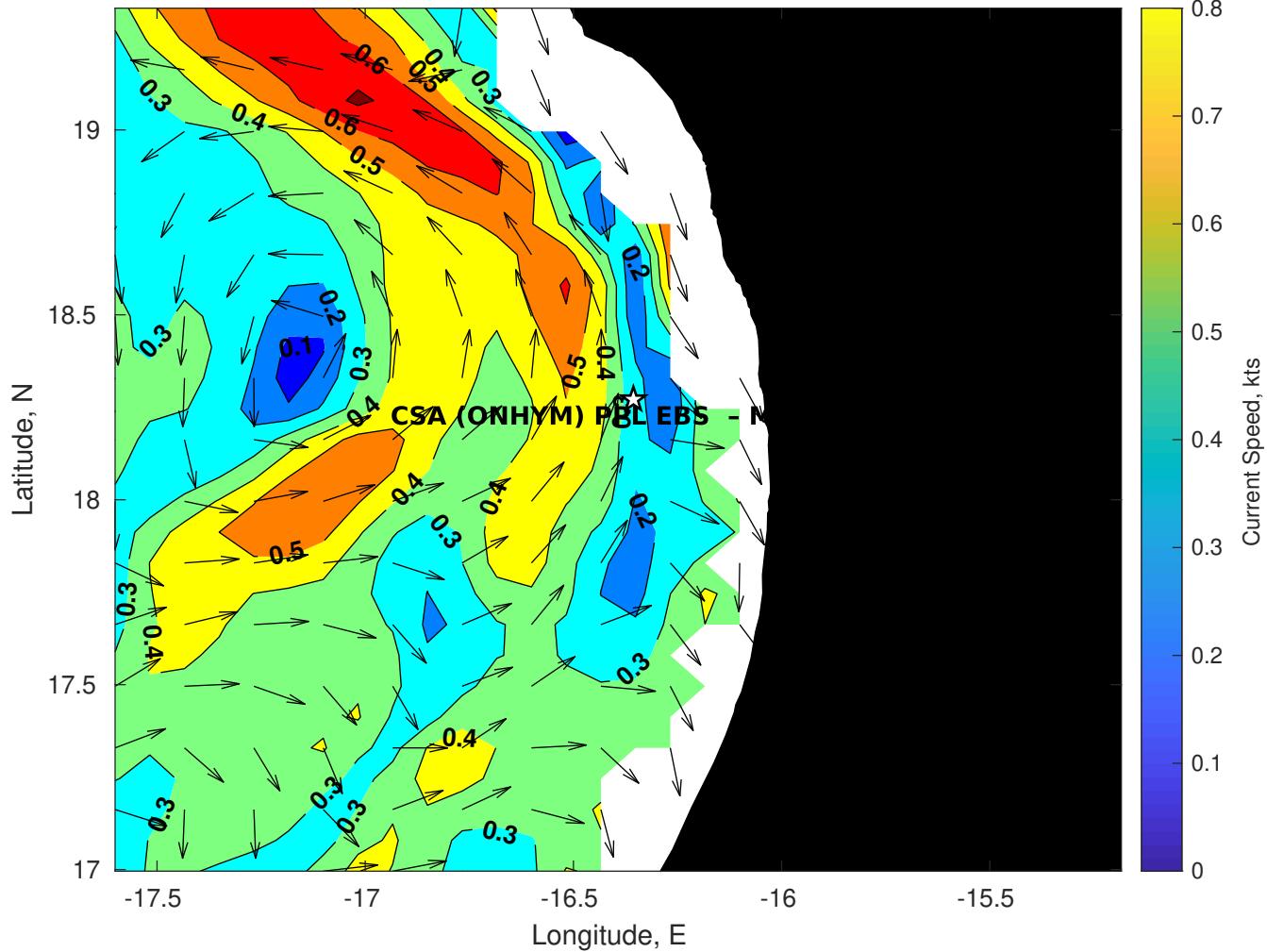
Surface Currents for CSA (ONHYM) PPL EBS - Mauritania at 24-Jul-2025 00:00:00
