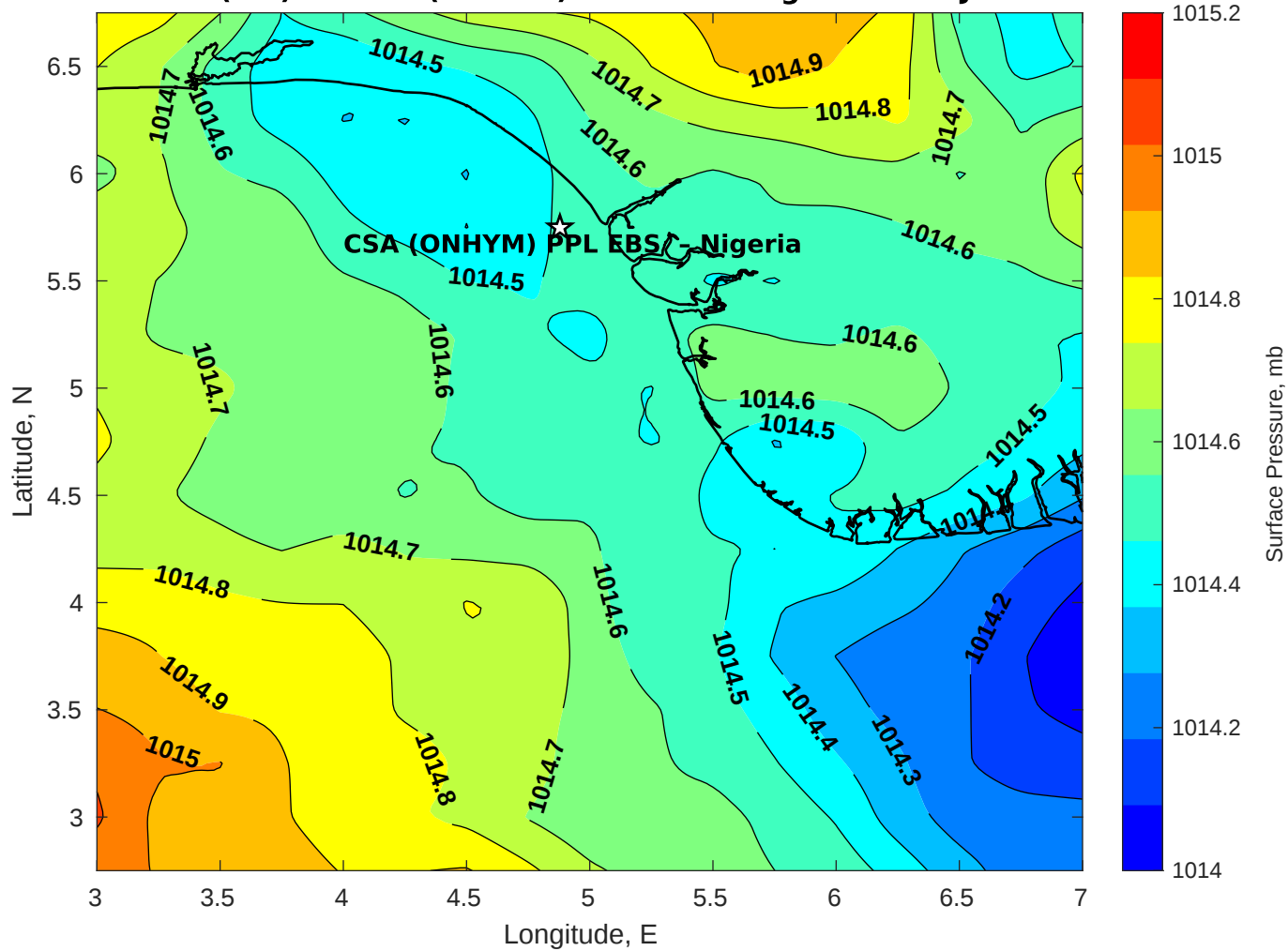
Surface Pressure (mb) for CSA (ONHYM) PPL EBS - Nigeria at 25-Jul-2025 00:00:00
