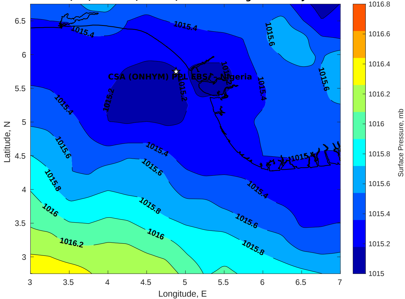
Surface Pressure (mb) for CSA (ONHYM) PPL EBS - Nigeria at 27-Jul-2025 00:00:00
