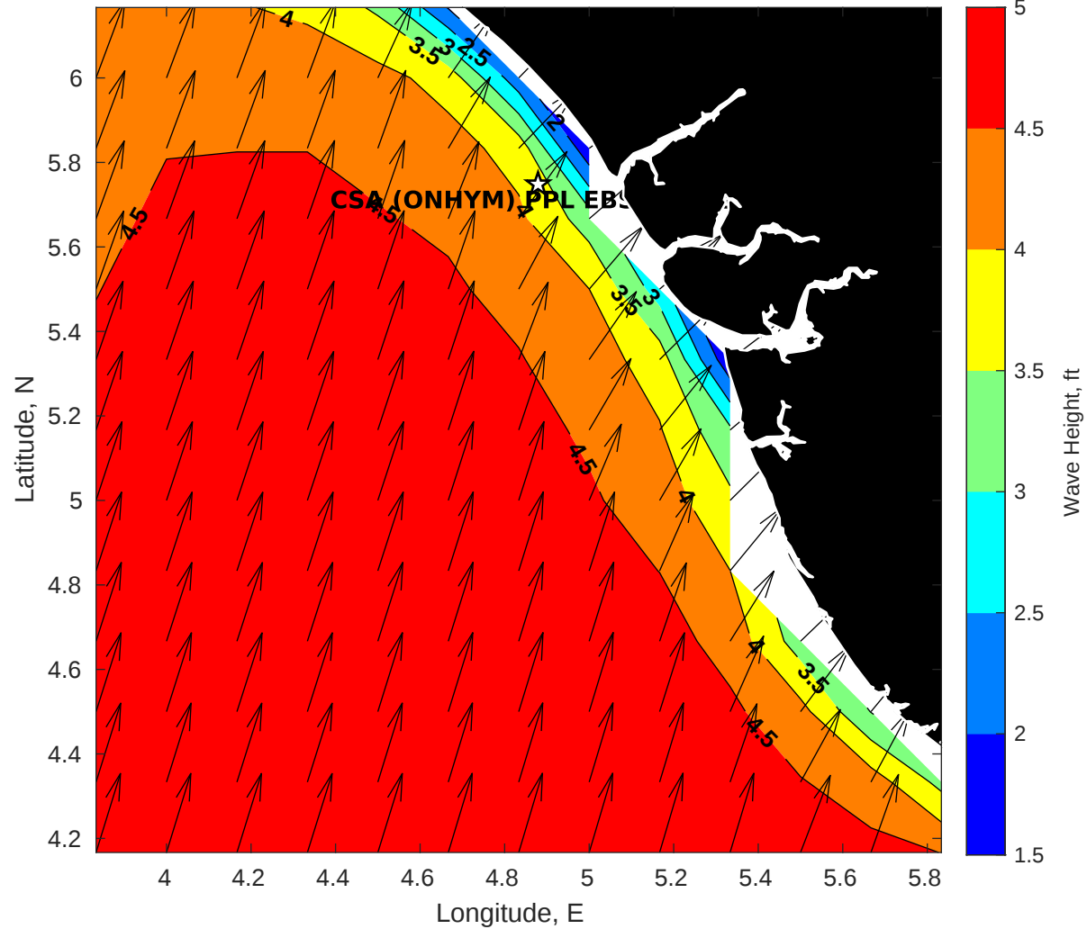
Wave Height (ft) for CSA (ONHYM) PPL EBS - Nigeria at 25-Jul-2025 09:00:00
