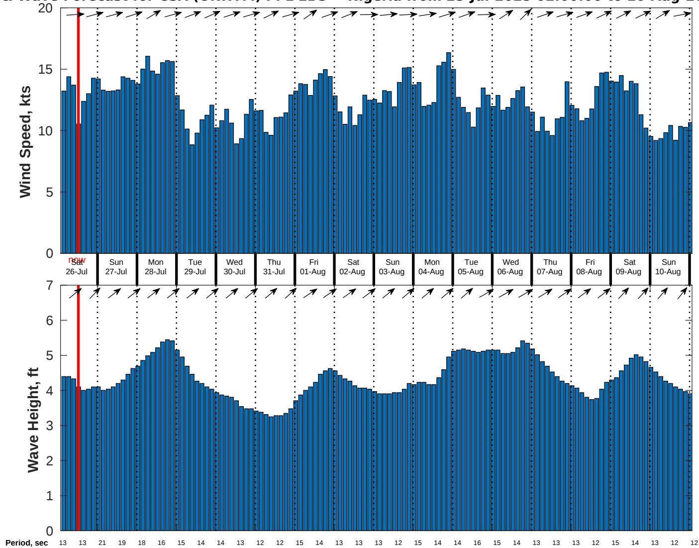
Wind & Wave Forecast for CSA (ONHYM) PPL EBS - Nigeria from 25-Jul-2025 02:00:00 to 10-Aug-2025 02:00:00
